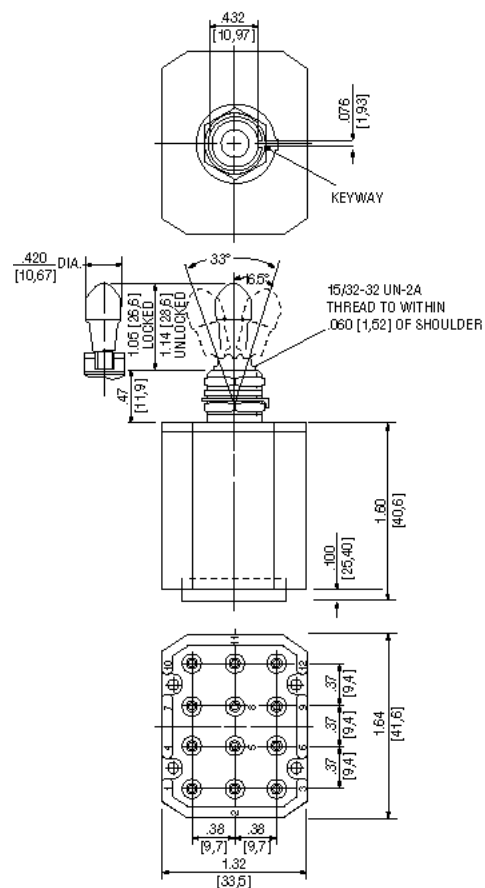
Terminal Identification
