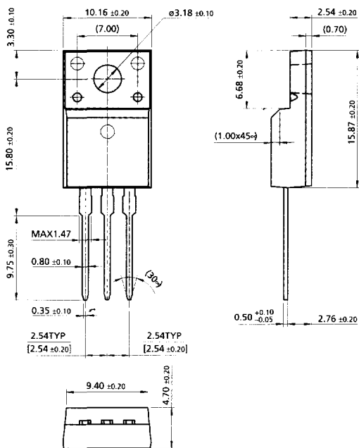
TO-220F (FS PKG Code AQ)
