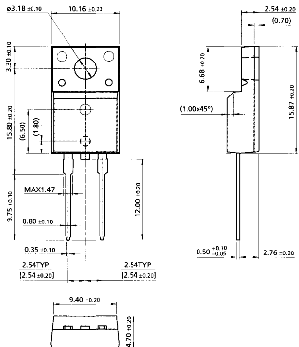
TO-220F-2L (FS PKG Code BL)
