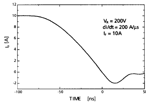
t rr Waveform of FFPF10U20S
