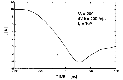
t rr Waveform of FFPF10U60S
