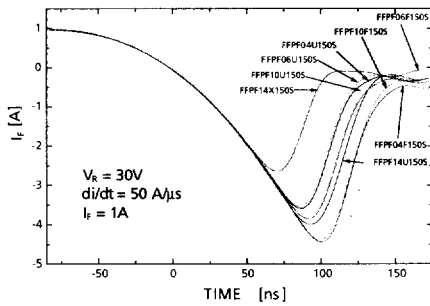
t rr Waveform of Damper Diode
