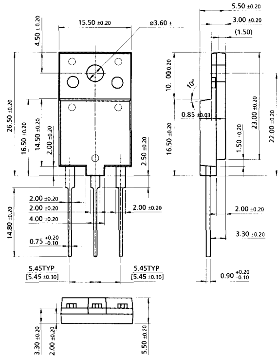
TO-3PF (FS PKG Code AG)
