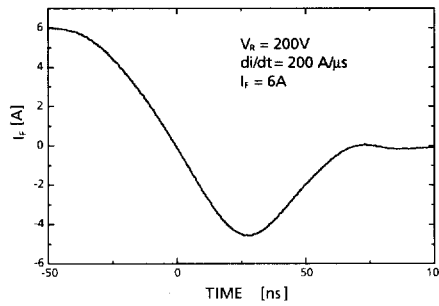
t rr Waveform of Modulation Diode
