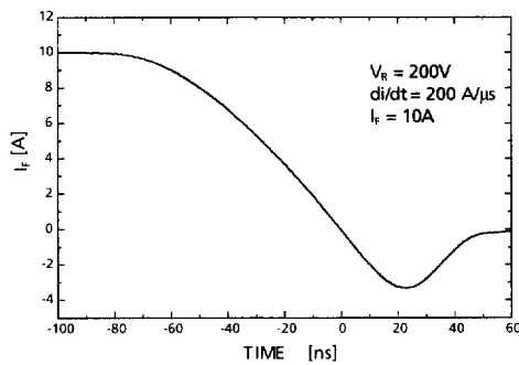
t rr Waveform of FFPF10U40S
