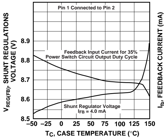
Figure 7. Feedback Input Shunt Regulation Voltage and Current vs. Temperature
