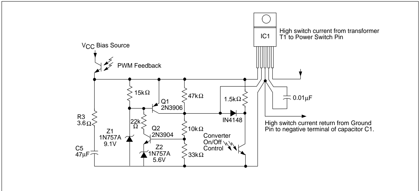
Figure 29. Converter Soft-Start
