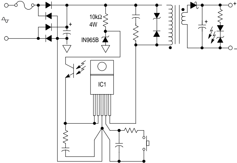
Figure 26. Transformer Auxiliary Winding Elimination Zener Shunt Regulator Method
