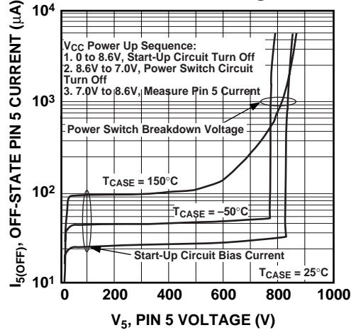
Figure 15. Power Switch Circuit Off-State Current vs. Voltage
