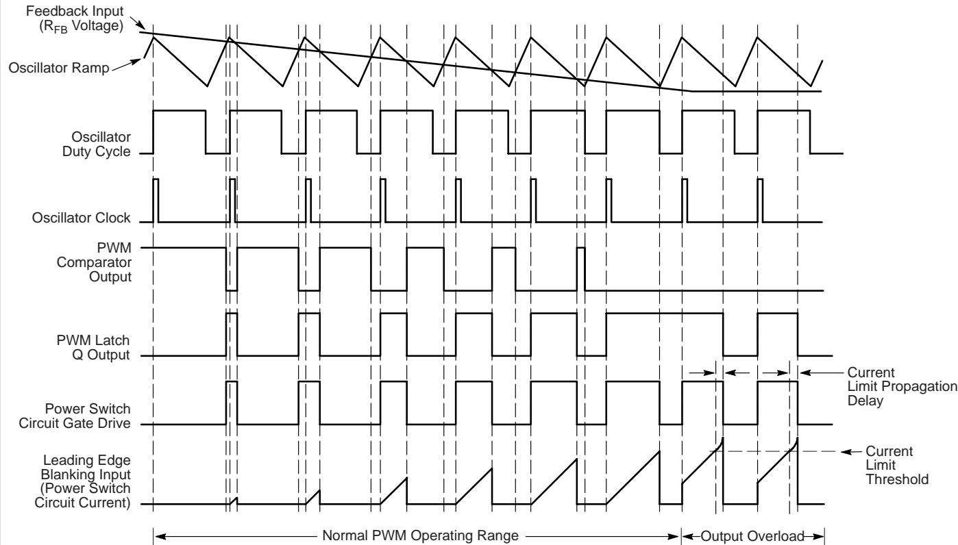
Figure 18. Pulse Width Modulation Timing Diagram
