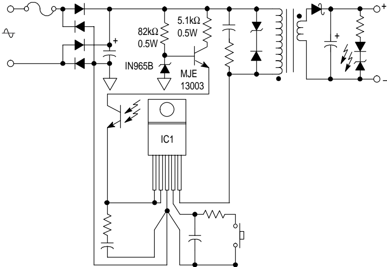
Figure 27. Transformer Auxiliary Winding Elimination Bipolar Transistor Series Regulator Method
