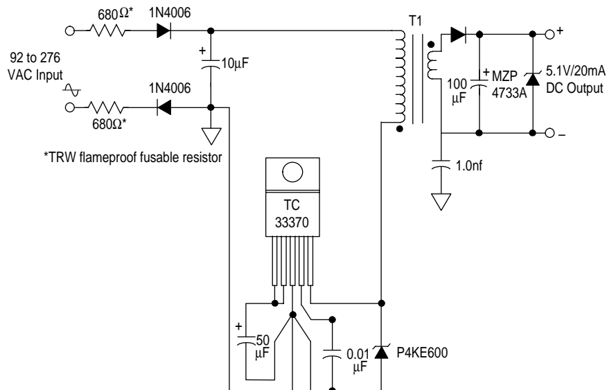
Figure 31. Low Power Off-Line Converter
