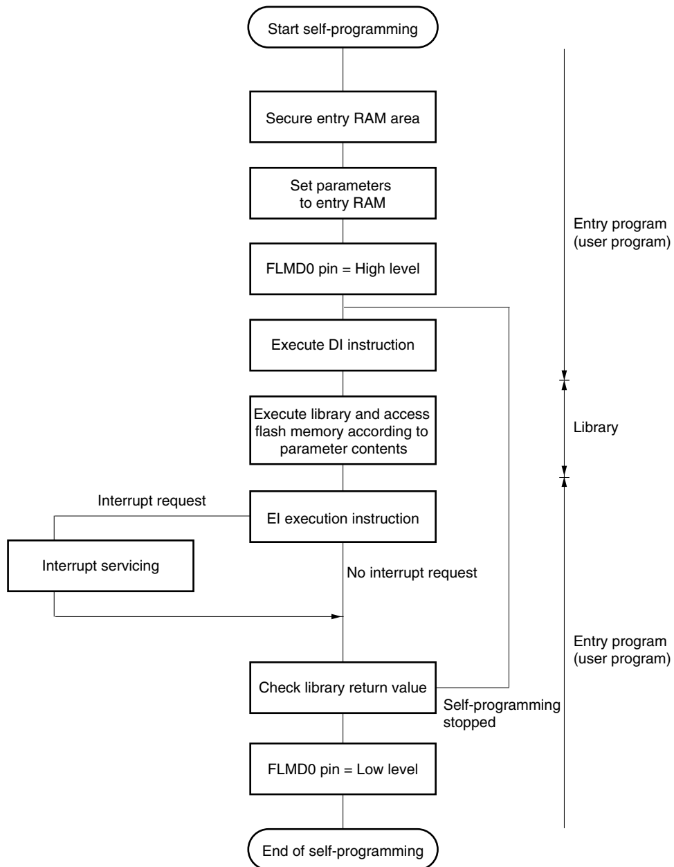
Figure 26-19. Self-Programming Procedure
