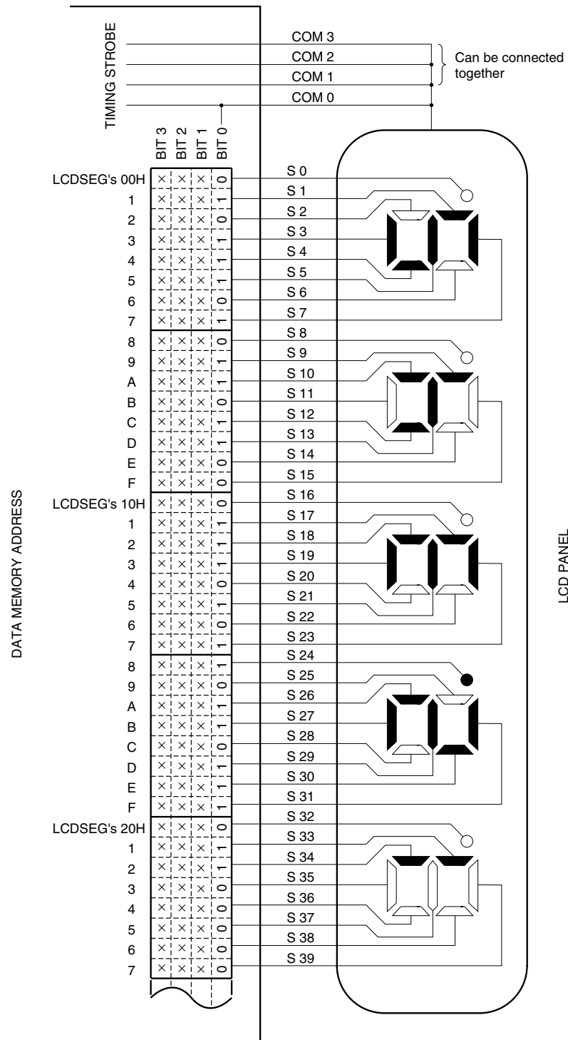
Figure 17-16. Example of Connecting Static LCD Panel
