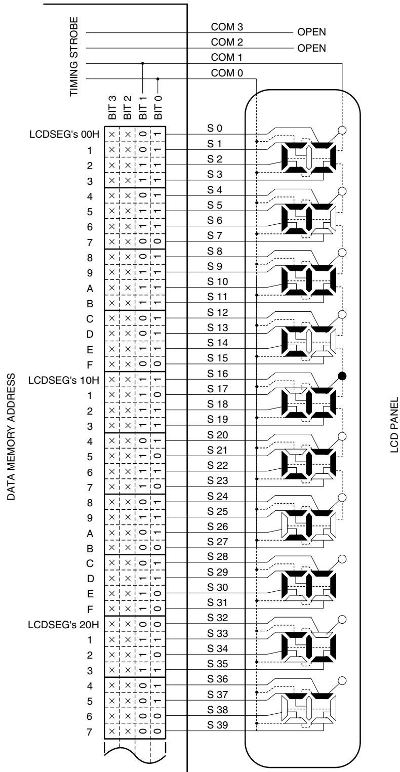
Figure 17-19. Example of Connecting Two-Time-Slice LCD Panel
