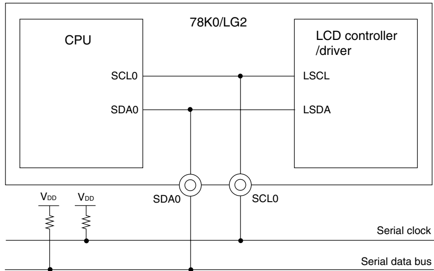
Figure 16-29. System configuration
