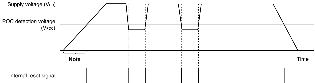
Figure 23-2. Timing of Internal Reset Signal Generation in Power-on-Clear Circuit
