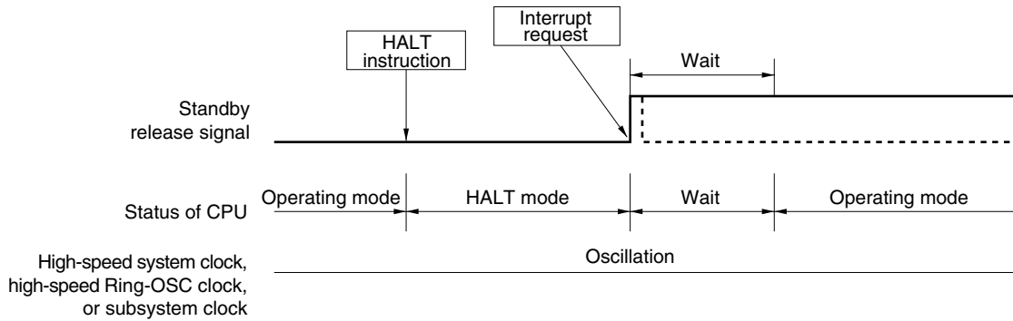
Figure 21-3. HALT Mode Release by Interrupt Request Generation
