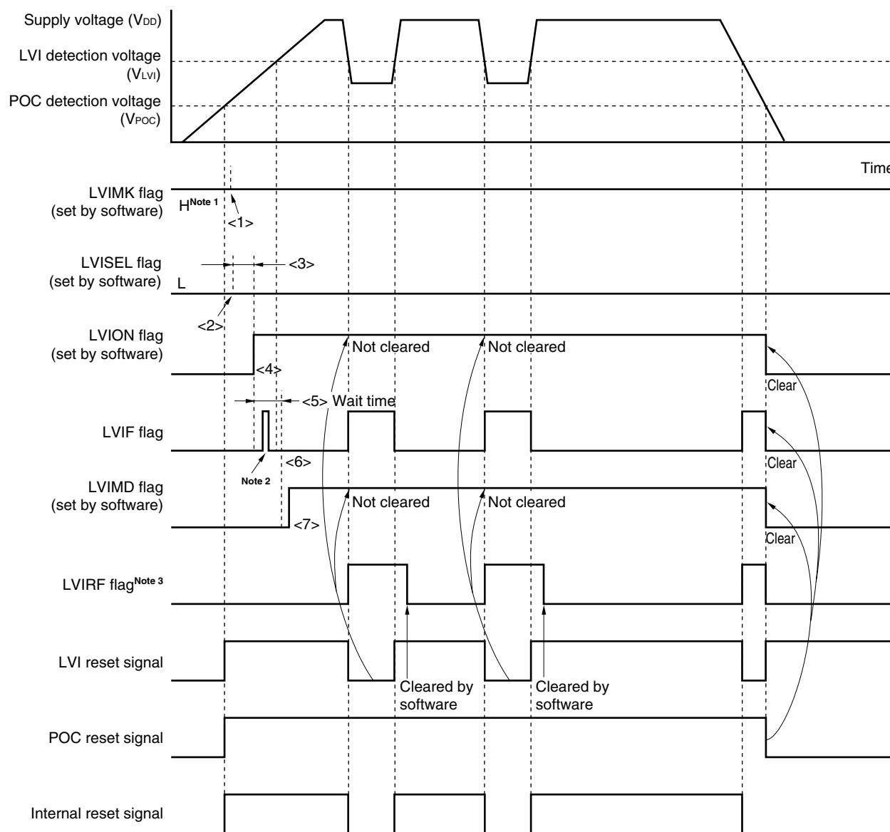
Figure 24-5. Timing of Low-Voltage Detector Internal Reset Signal Generation (Detects Level of Supply Voltage ( V_{DD} ))
