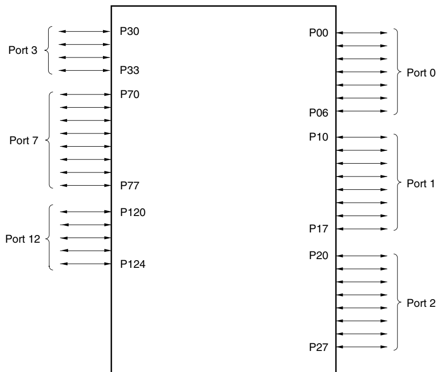
Figure 4-1. Port Types
