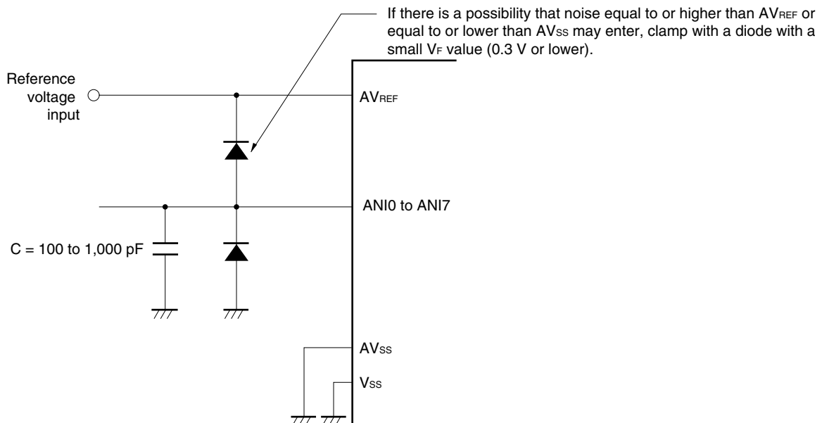
Figure 12-20. Analog Input Pin Connection
