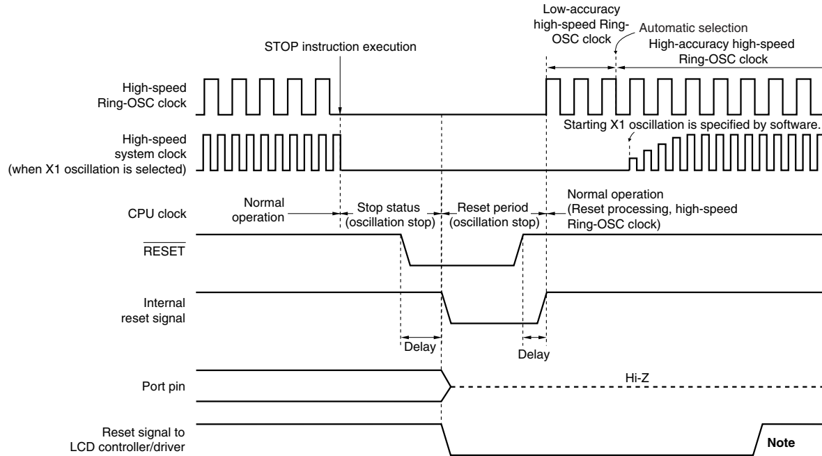
Figure 22-4. Timing of Reset in STOP Mode by \overline{\text{RESET}} Input
