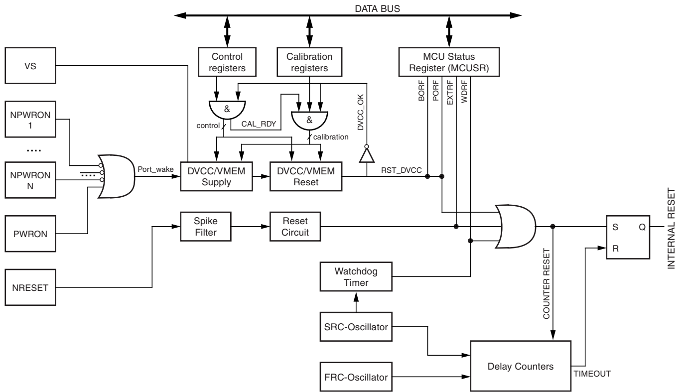
Figure 4-4. Reset Logic
