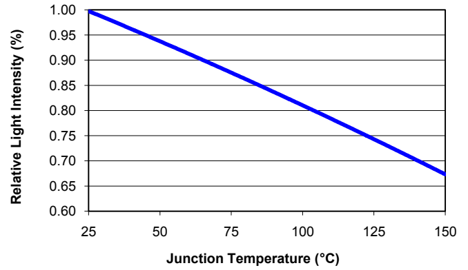
Relative Light Intensity vs. Junction Temperature
