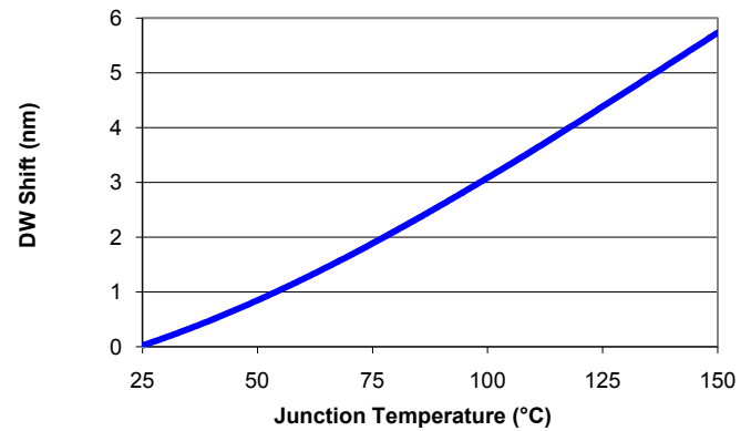
Dominant Wavelength Shift vs. Junction Temperature
