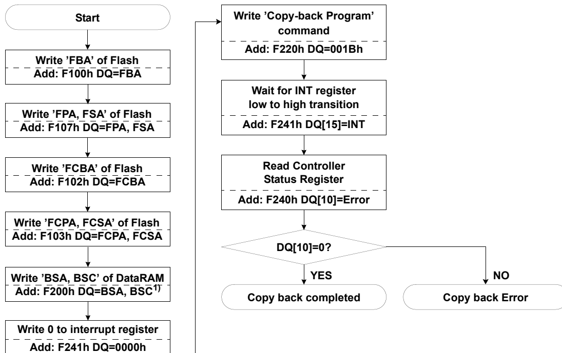
Copy-Back Program Operation Flow Chart
