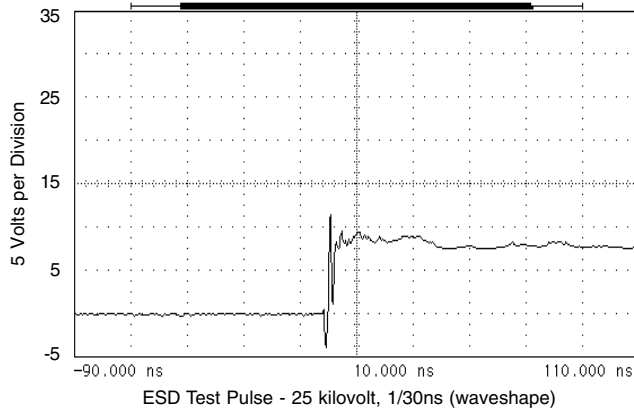
FIGURE 4 OVERSHOOT & CLAMPING VOLTAGE FOR LC0404FC05C
