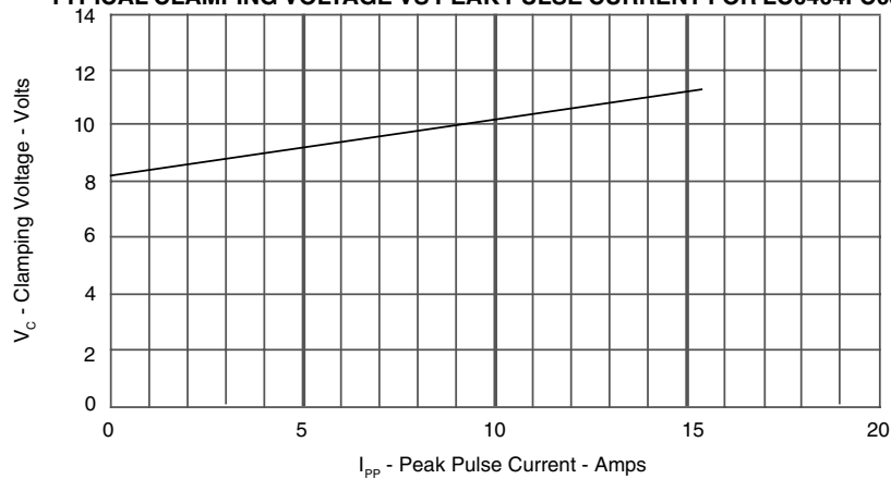
FIGURE 5 TYPICAL CLAMPING VOLTAGE VS PEAK PULSE CURRENT FOR LC0404FC05C
