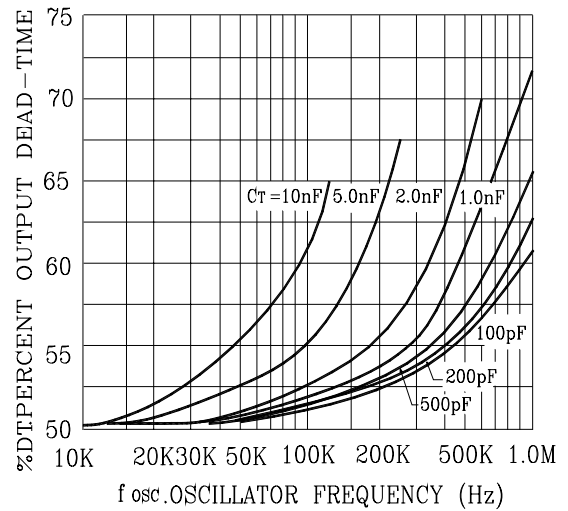
FIGURE 2-OUTPUT DEAD TIME versus OSCILLATOR FREQUENCY
