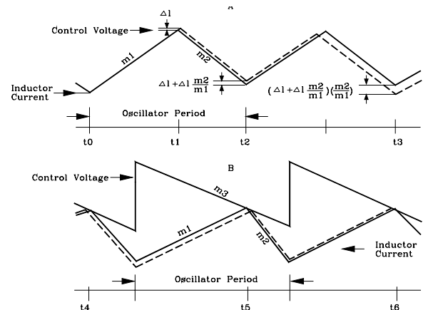
FIGURE 19-CONTINUOUS CURRENT WAVEFORMS
