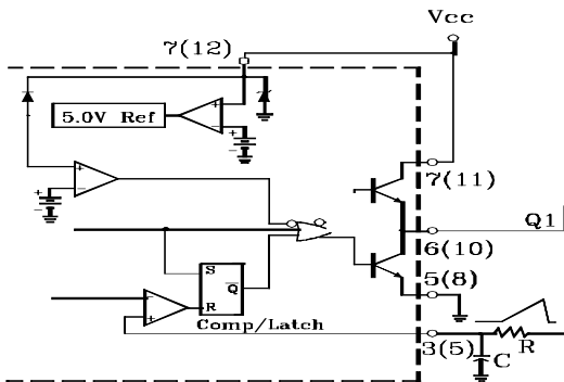
FIGURE 26-CURRENT WAVEFORM SPIKE SUPPRESSION
