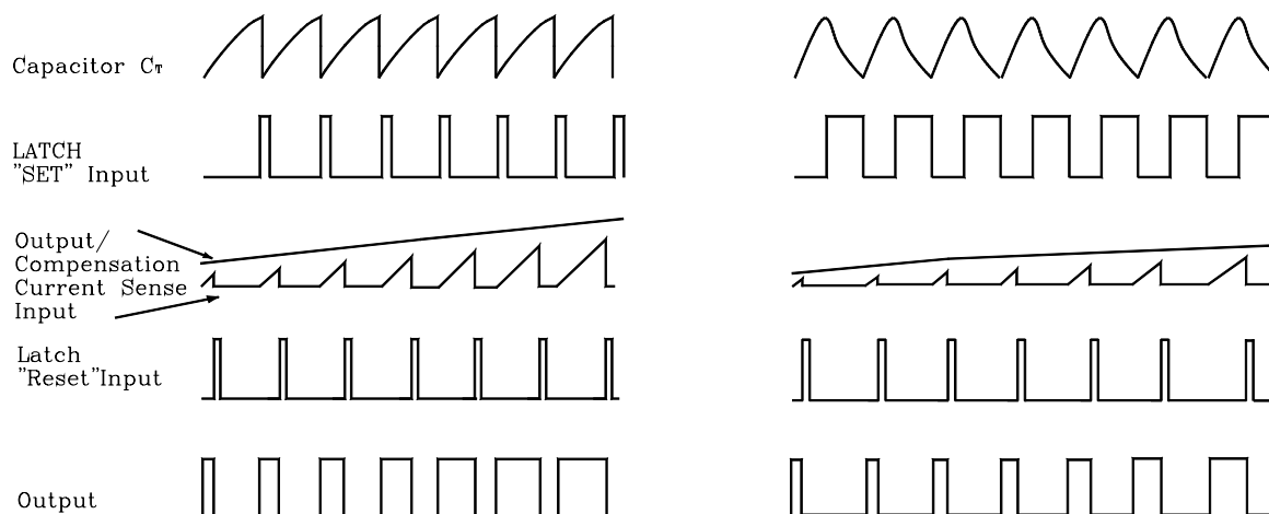
FIGURE 18-TIMING DIAGRAM
