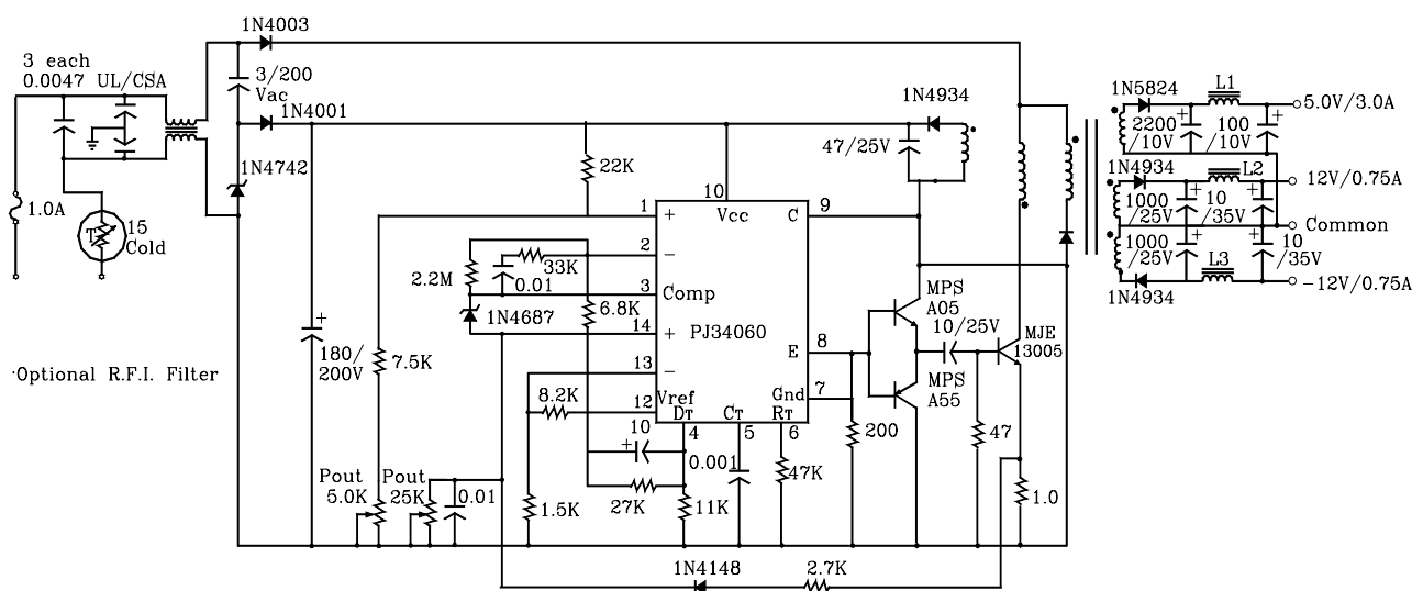
FIGURE 21-33 WATT OFF-LINE FLYBACK CONVERTER WITH SOFT-START AND PRIMARY POWER LIMITING
