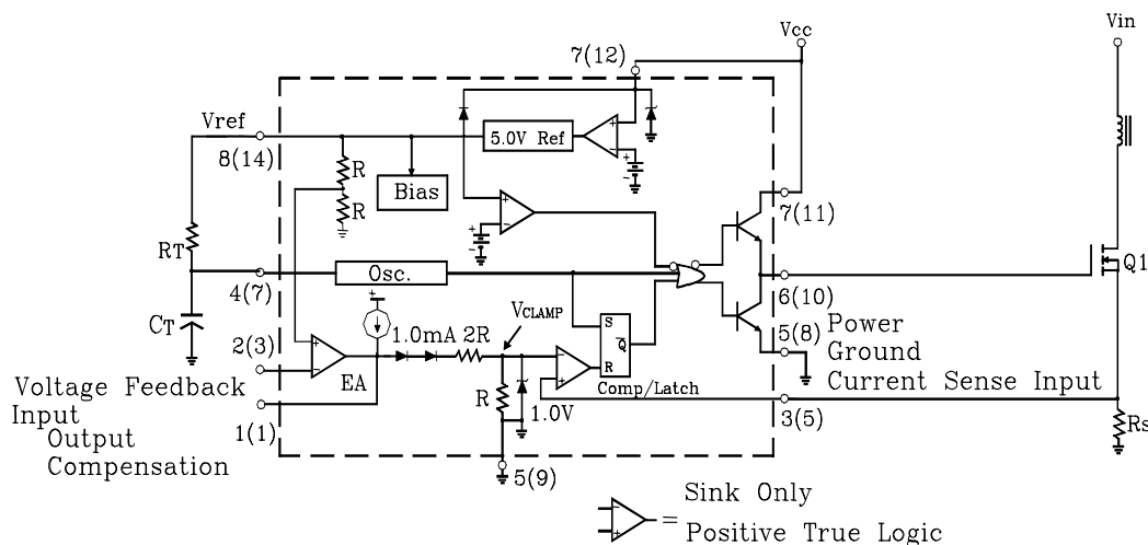
FIGURE 17-REPRESENTATIVE BLOCK DIAGRAM
