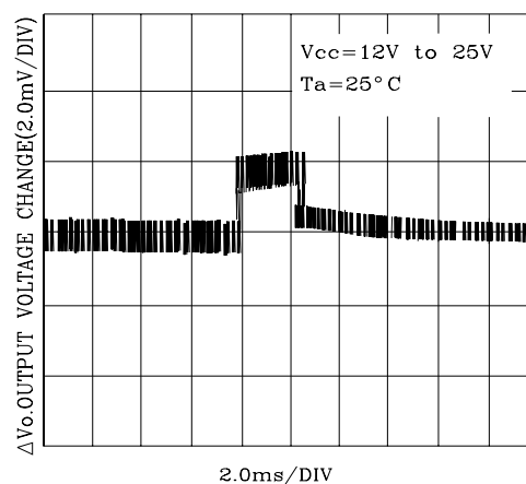
FIGURE 12-OUTPUT WAVEFORM
