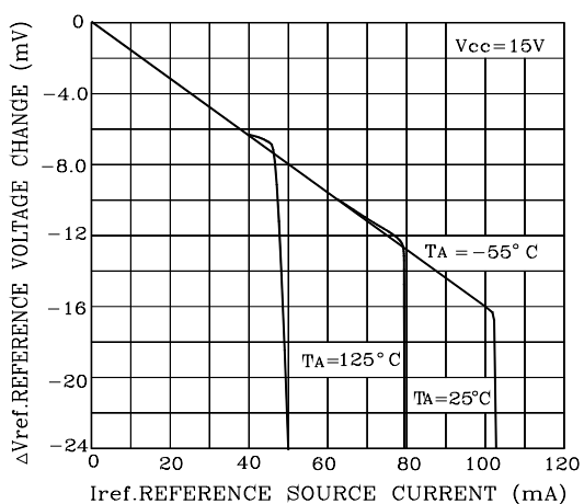
FIGURE 9-REFERENCE LOAD REGULATION
