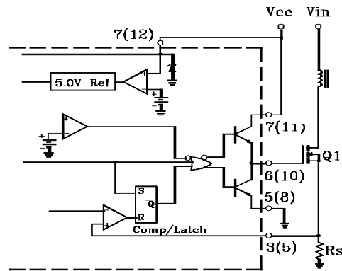
FIGURE 27-MOSFET PARASITIC OSCILLATIONS
