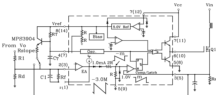
FIGURE 32-SLOPE COMPENSATION
