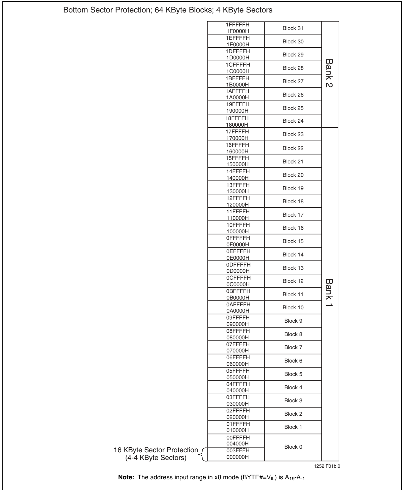
FIGURE 2: SST34HF16x1S, 2M x8 CONCURRENT SUPERFLASH DUAL-BANK MEMORY ORGANIZATION
