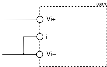
Fig. 23 If the inhibit is not used the inhibit pin should be connected to Vi-
