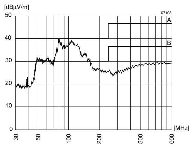
Fig. 17 Typical radio frequency-interference voltage at U_{i\text{ nom}} , I_{o\text{ nom}} , measured with an antenna (distance 10 m). Output leads 1 m, twisted.
