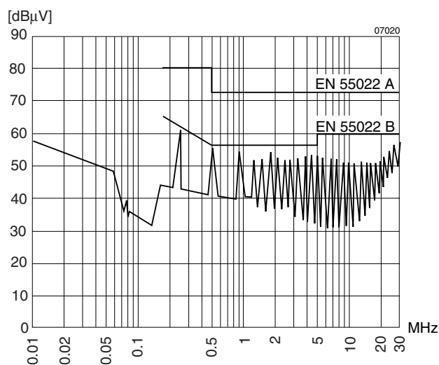
Fig. 16 Typical disturbance voltage (quasi-peak) at the input according to CISPR 11/EN 55011 and CISPR 22/EN 55022, measured at U_{i\text{ nom}} and I_{o\text{ nom}} . Output leads 0.1 m, twisted. (48 IMS 15-05)
