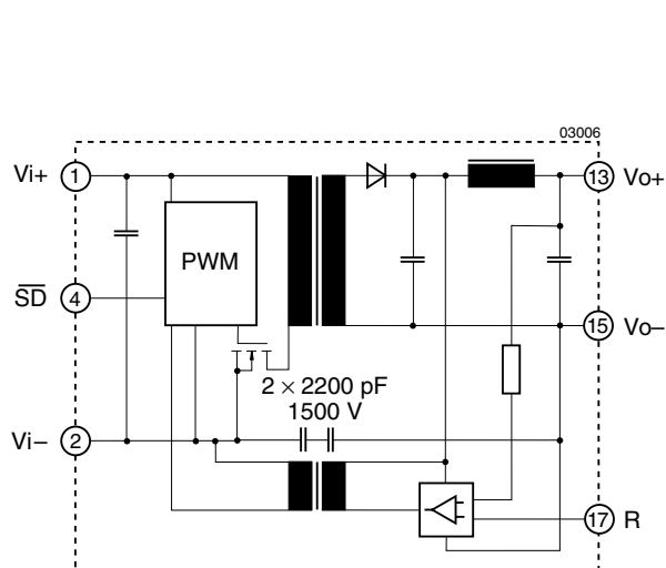
Fig. 1 Block diagram, single output types.
