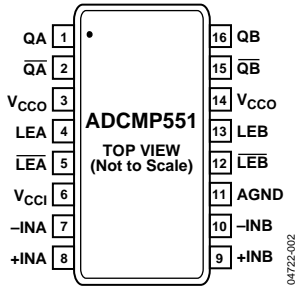
Figure 2. ADCMP551 16-Lead QSOP Pin Configuration
