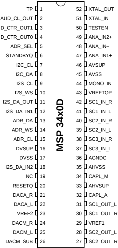
Fig. 9–8: 52-pin PSDIP package
