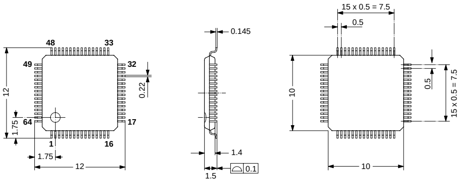
Fig. 9-5: 64-Pin Plastic Low-Profile Quad Flat Pack (PLQFP64) Weight approximately 0.35 g Dimensions in mm
