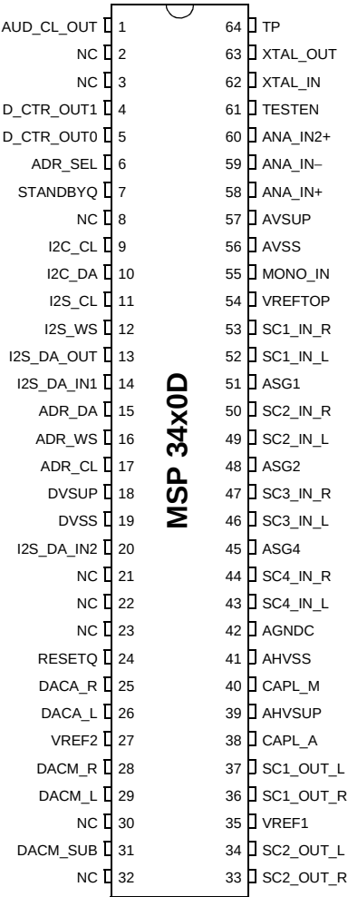
Fig. 9–7: 64-pin PSDIP package
