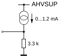
Fig. 9-20: Output Pins 56, 57, 59, 60, and 54 (DACA_L/R, DACM_L/R, DACM_SUB)
