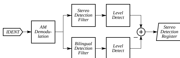
Fig. 4–4: Stereo/bilingual detection
