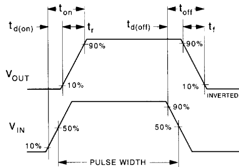
Figure 12. Switching Waveforms.
