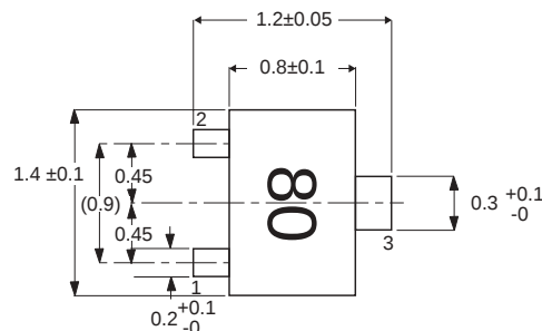
PACKAGE OUTLINE M03
