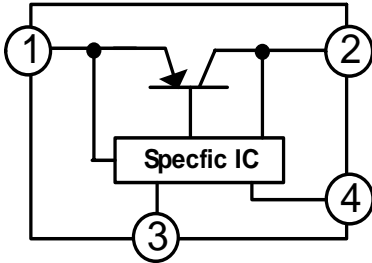
TO-220F-4
