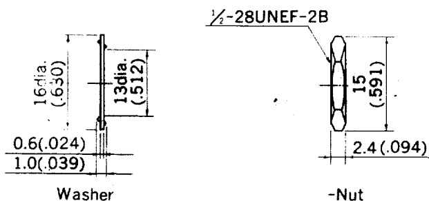
Mounting washer and nut
