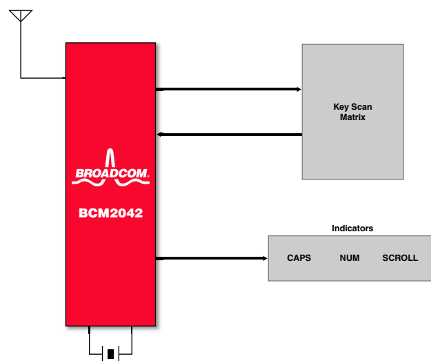
BCM2042 Keyboard Block Diagram
