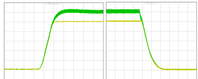
Figure 36: Sequential Start-up
