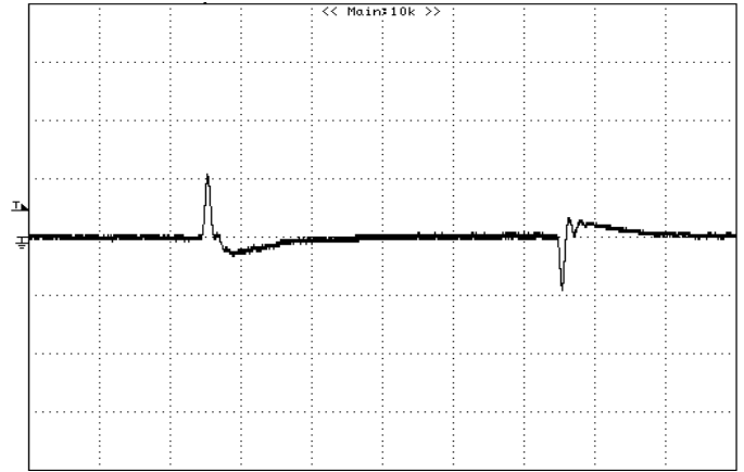
Figure 36: Typical transient response to step load change at 1A/\mu S from 0%~ 50%~0% of I_o , max at 12Vin, 5.0Vout (Cout = 1uF ceramic, 47uF+10uFceramic) CH1 : VOUT, 0.2V/div, 100uS/div
