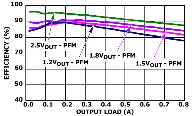
FIGURE 3. EFFICIENCY vs LOAD 2.25MHz 3.3VIN PFM
