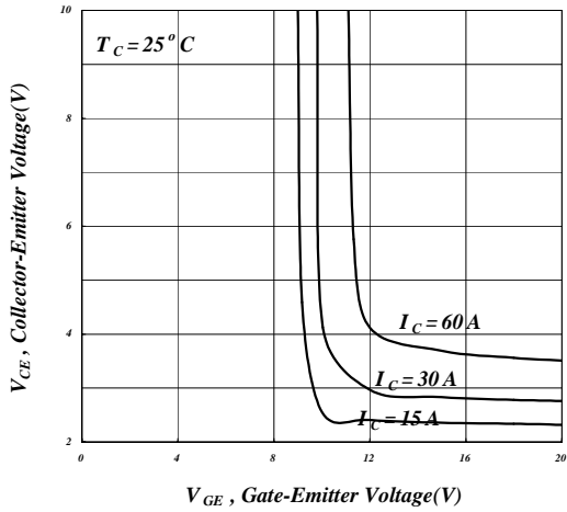
Fig 9. Saturation Voltage vs. V_{GE}
