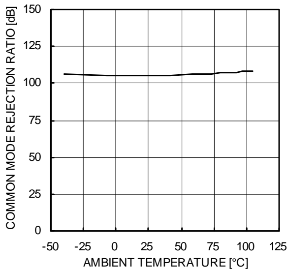
Fig.83 Common Mode Rejection Ratio - Ambient Temperature (VCC/VEE=+15V/-15V, Vicm=-12V to +12V)
