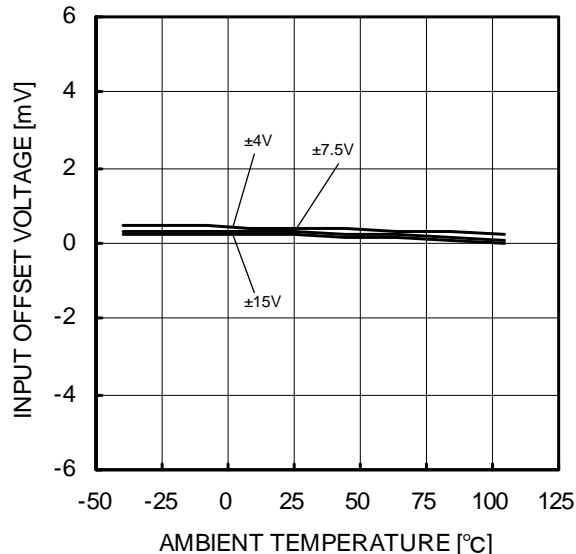
Fig.77 Input Offset Voltage - Ambient Temperature (Vicm=0V, Vout=0V)
