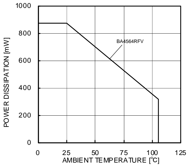
Fig.46 Derating Curve
