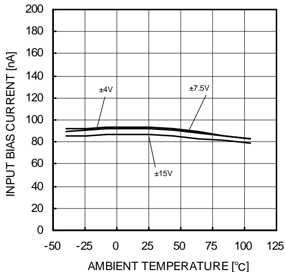
Fig.79 Input Bias Current - Ambient Temperature (Vicm=0V, Vout=0V)
