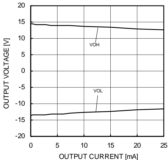
Fig.53 Maximum Output Voltage - Output Current (VCC/VEE=+15V/-15V, Ta=25°C)
