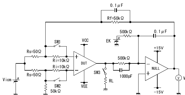
Fig. 90 Test circuit1 (one channel only)
