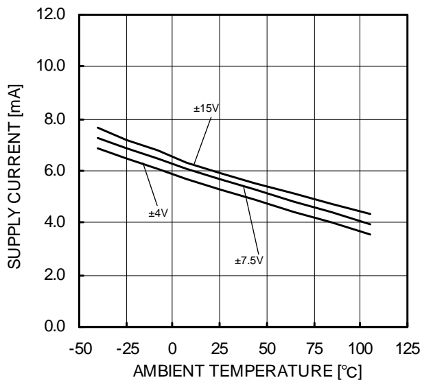
Fig.70 Supply Current - Ambient Temperature
