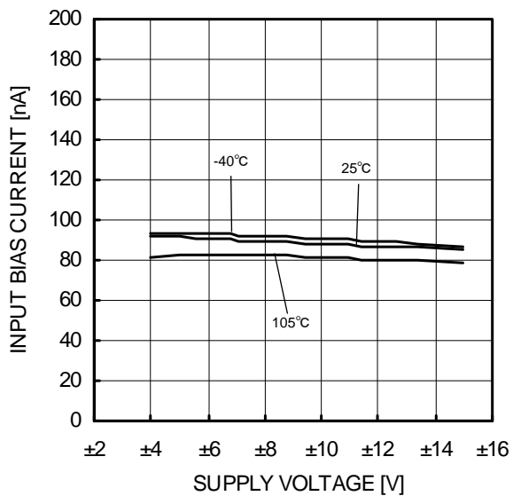
Fig.78 Input Bias Current - Supply Voltage (Vicm=0V, Vout=0V)
