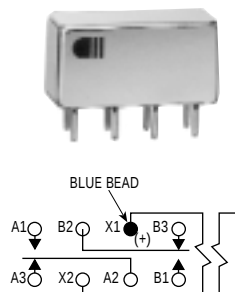
TERMINAL VIEW
