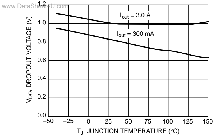
Figure 1. Dropout Voltage vs. Temperature
