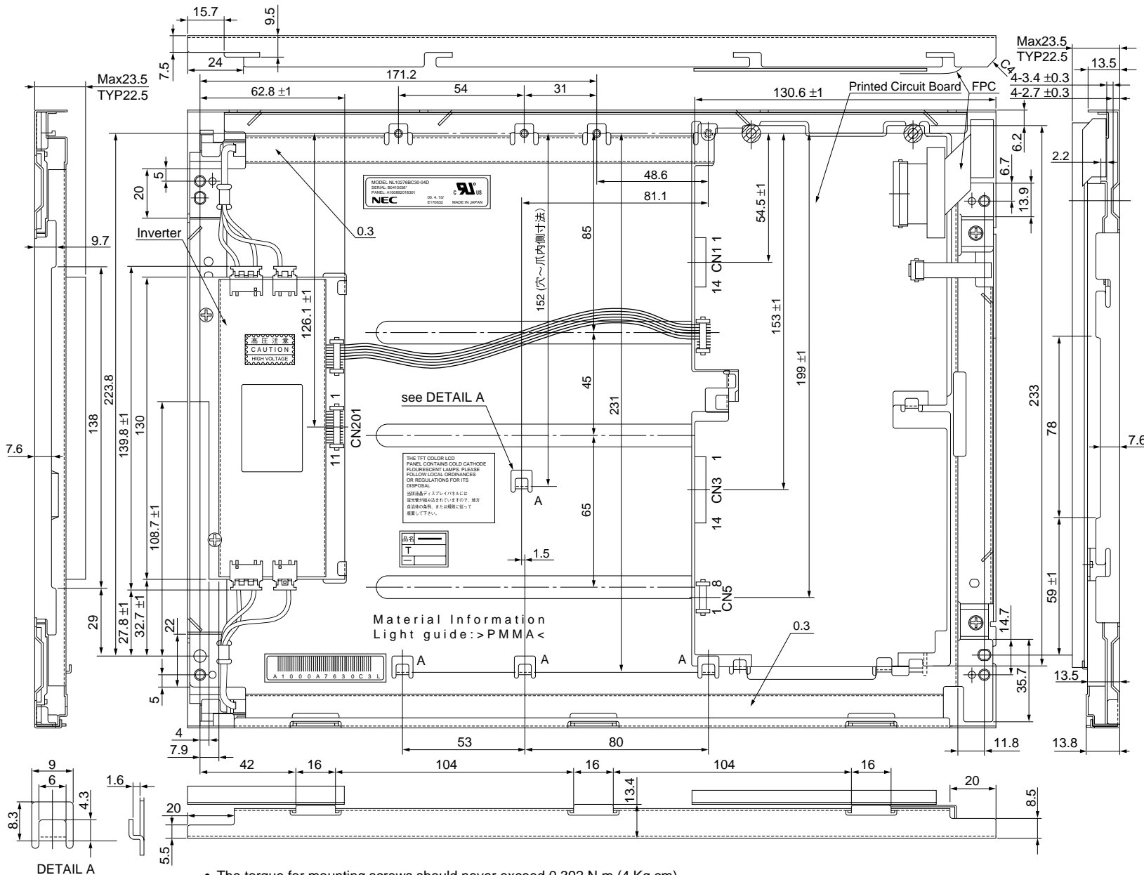
Rear View (Unit in mm)
