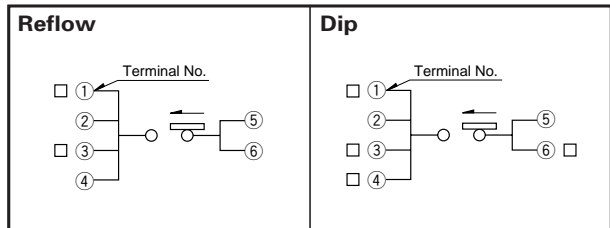
Circuit Diagram
