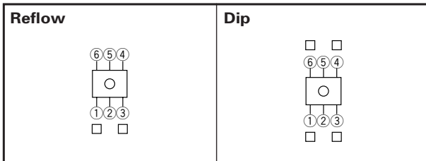
Terminal arrangement (Viewed from direction A)
