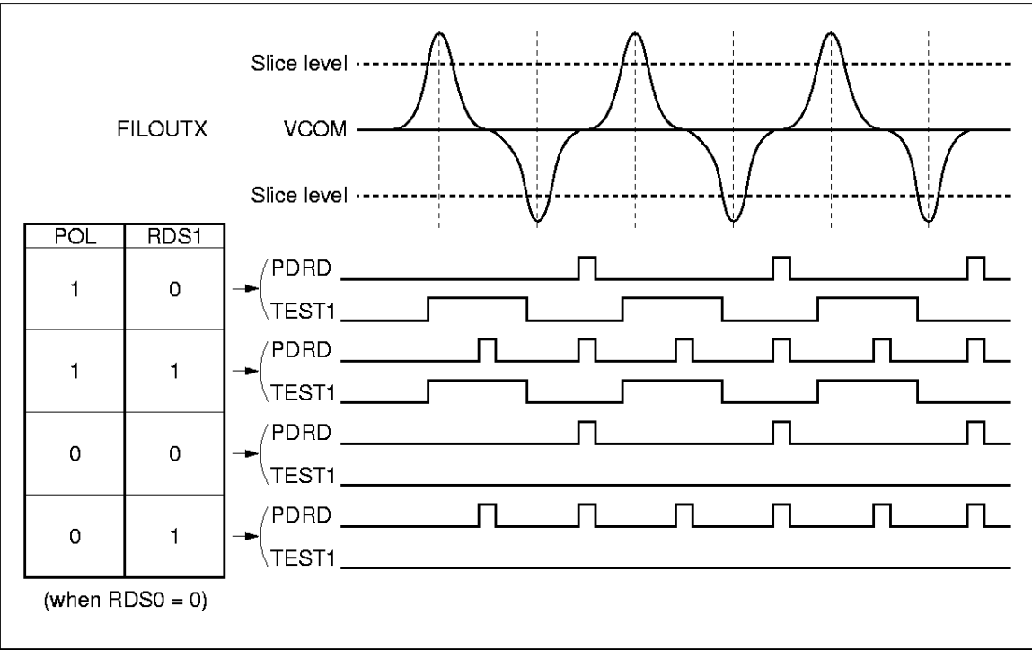
Figure 6 Polarity Signal Generate Function
