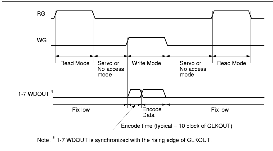
Figure 16 Read and Write Mode Timing
