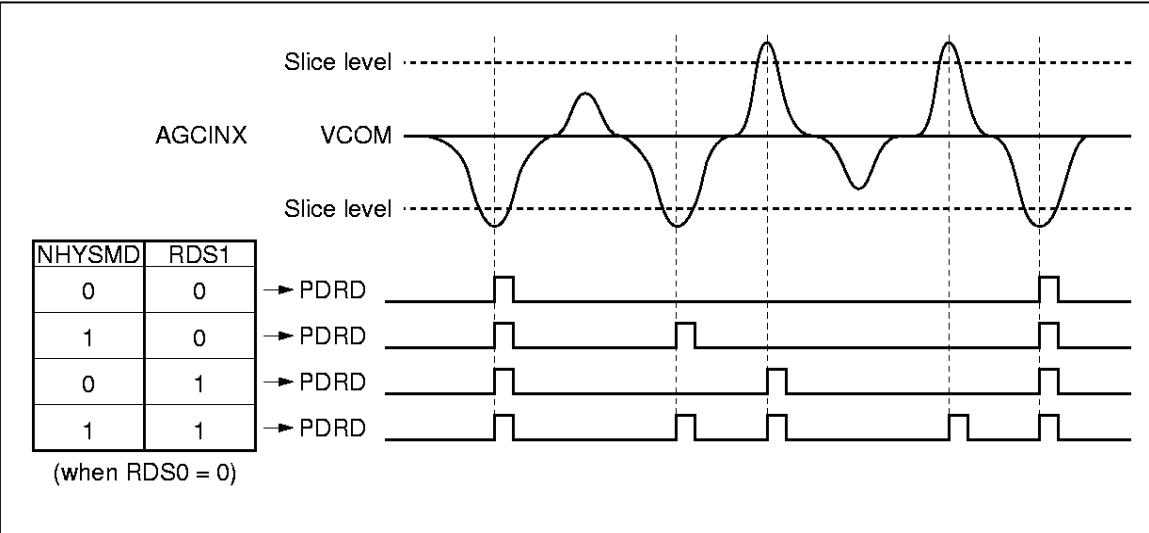
Figure 5 PDRD Pulse Generate Function
