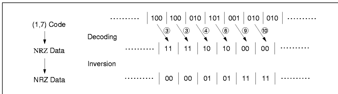
Figure 12 (1, 7) Code to NRZ Decoding Example
