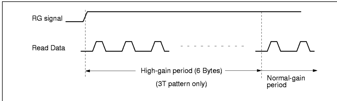
Figure 15 Sync Field Detection Timing
