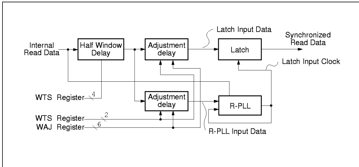
Figure 13 Window Adjustment Circuit Block Diagram
