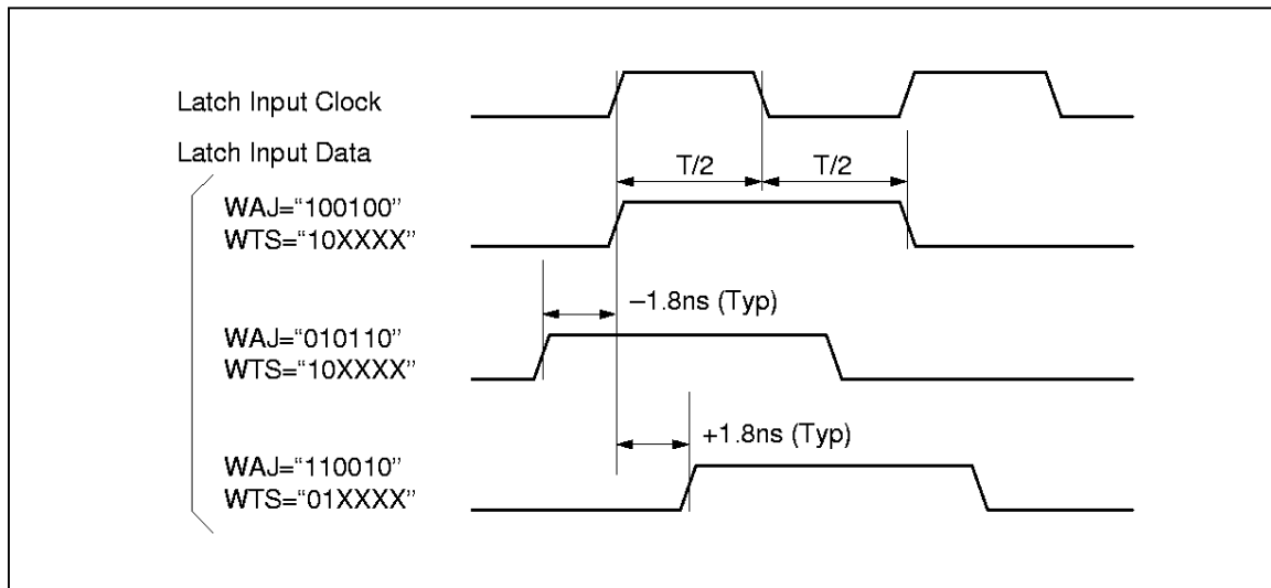
Figure 14 Window Adjustment Timing Waveform
