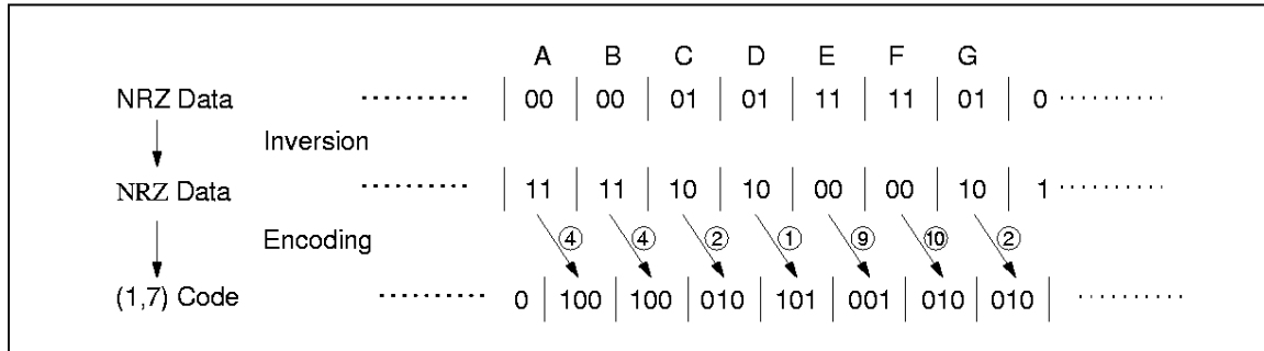
Figure 11 Shows an Example of NRZ to (1, 7) Code Conversion
