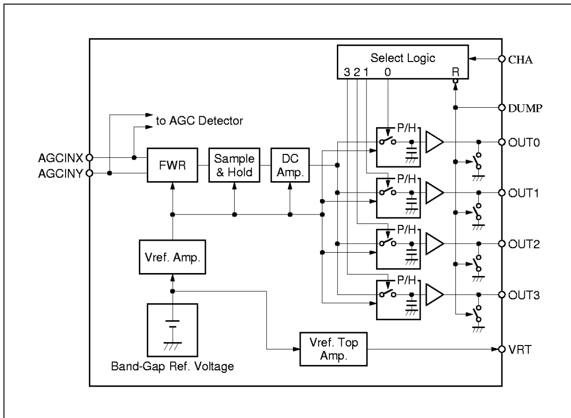
Figure 7 Servo Peak & Hold Circuit Block Diagram
