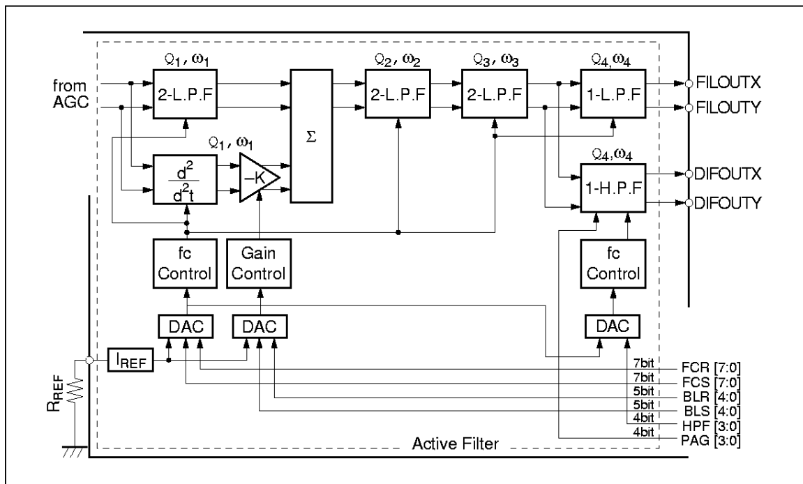
Figure 10 Active Filter Block Diagram
