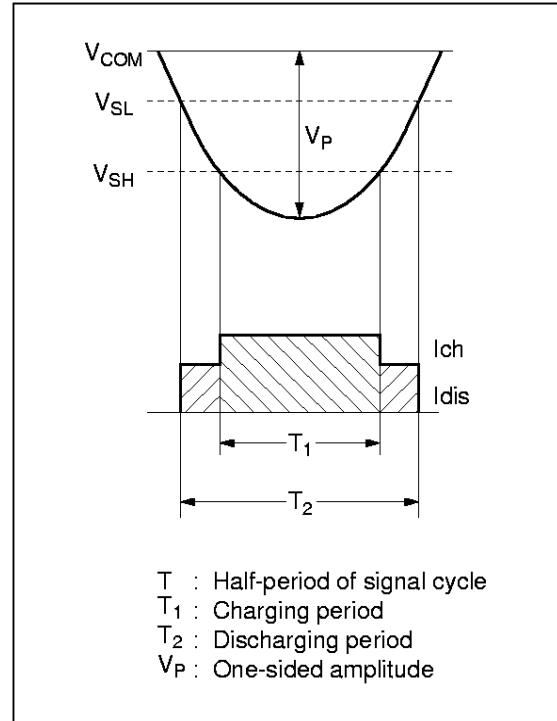
Figure 9 Charge / Discharge Timing
