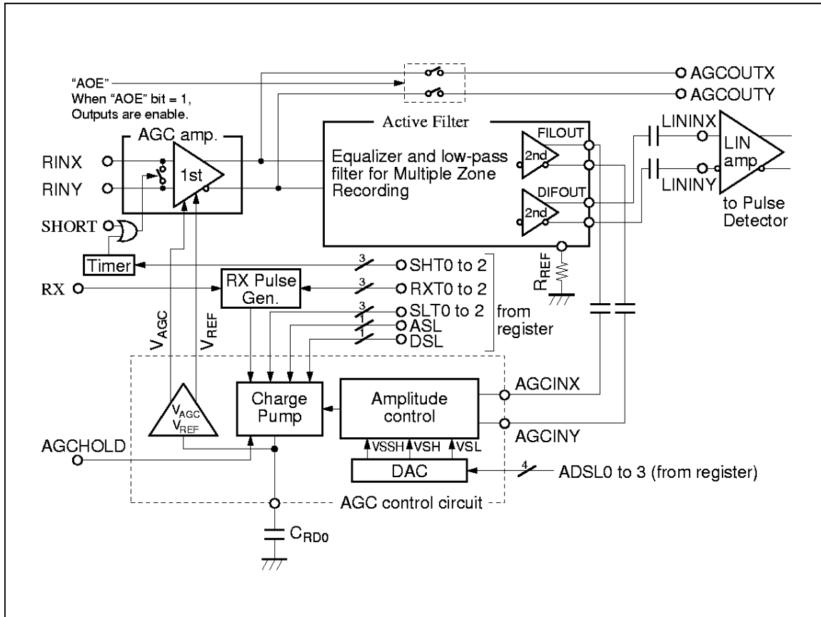
Figure 8 AGC Block Diagram
