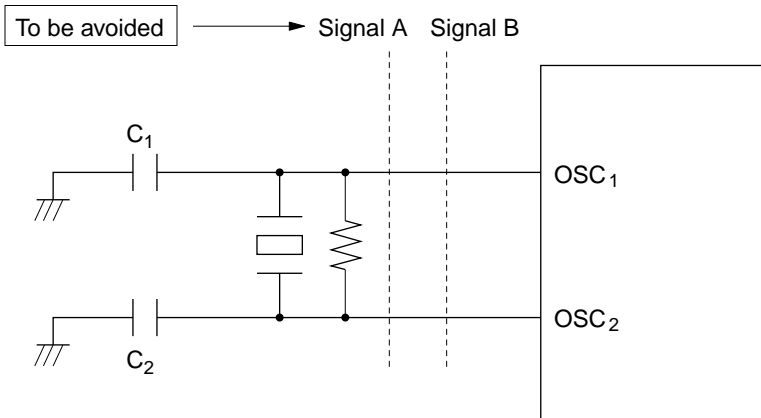
Figure 4.5 Board Design of Oscillator Circuit
