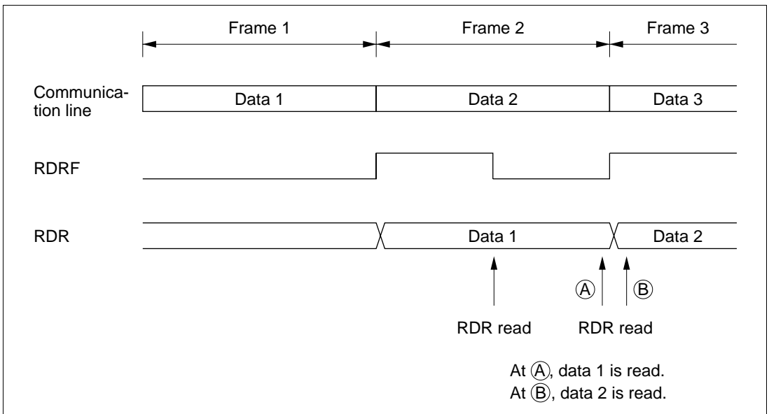
Figure 10.28 Relationship between Data and RDR Read Timing
