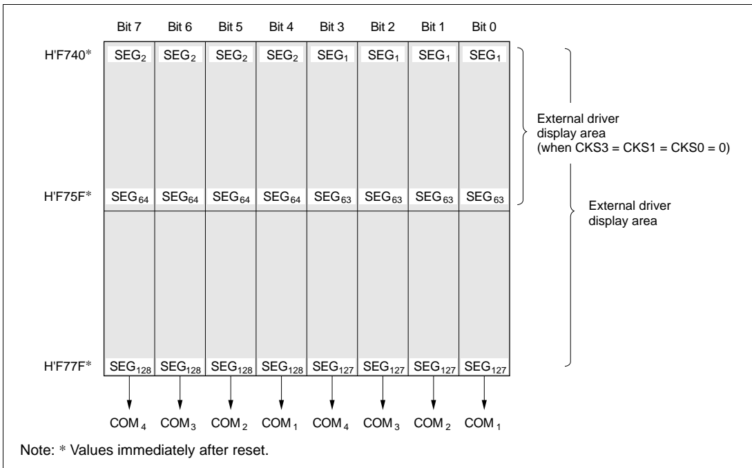
Figure 13.11 LCD RAM Map When All External Segments are Used (Example: SGX = 1, SGS3 to SGS0 = 0000, 1/4 Duty)
