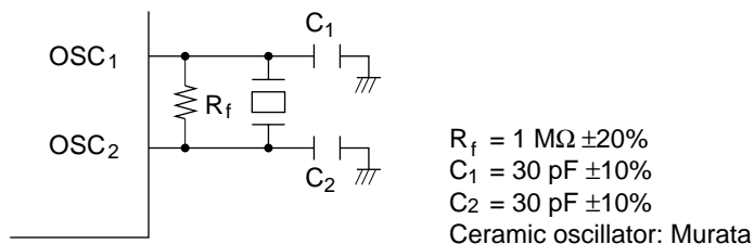
Figure 4.4 Typical Connection to Ceramic Oscillator
