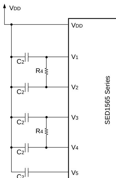
Exemplary connection diagram 2.
