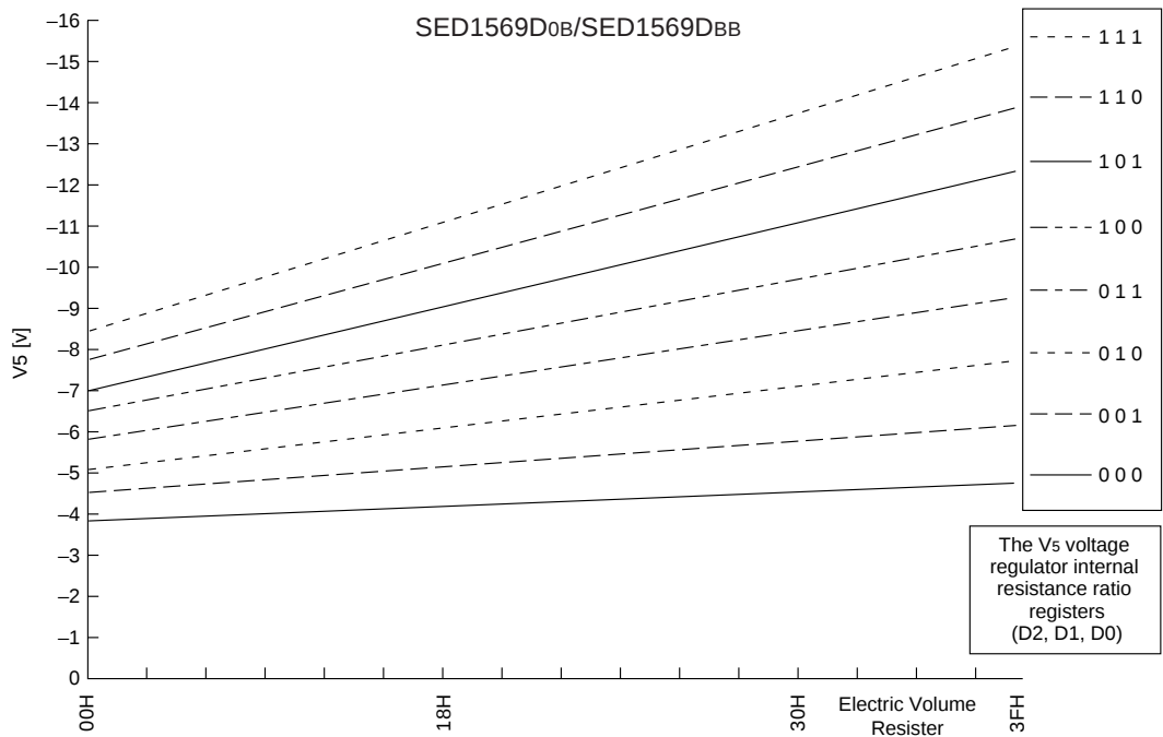
Figure 19: SED1569D0B/SED1569DDB (Temperature Gradient = -0.05\%/^{\circ}\text{C} Model)
