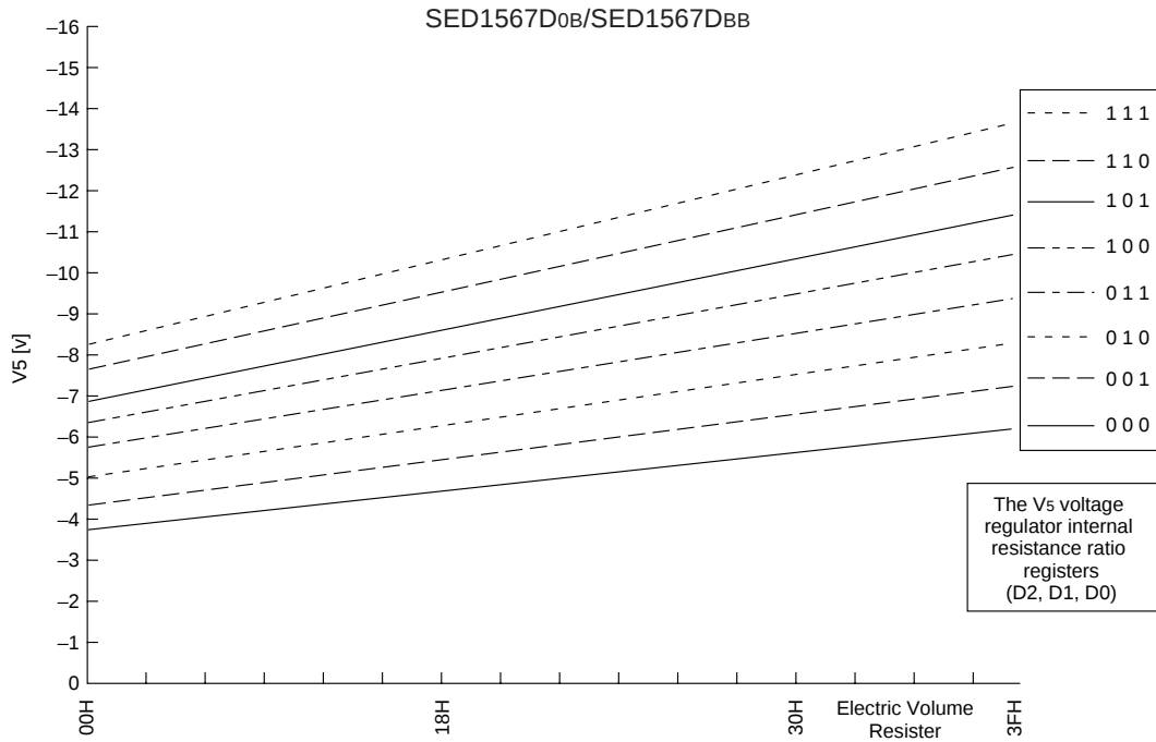
Figure 15: SED1567D0B/SED1567D0B (1) For Models Where the Thermal Gradient = -0.05\%/^{\circ}\text{C}
