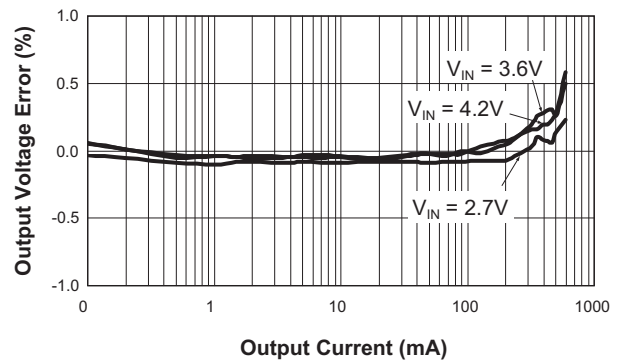
Load Regulation (LL Mode; V_{OUT} = 1.8V )
