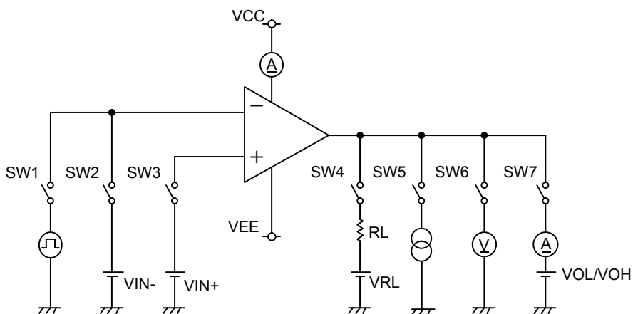
Fig.112 Test Circuit 2 (one channel only)
