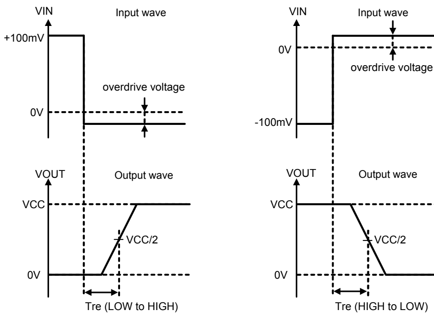
Fig.113 Response Time
