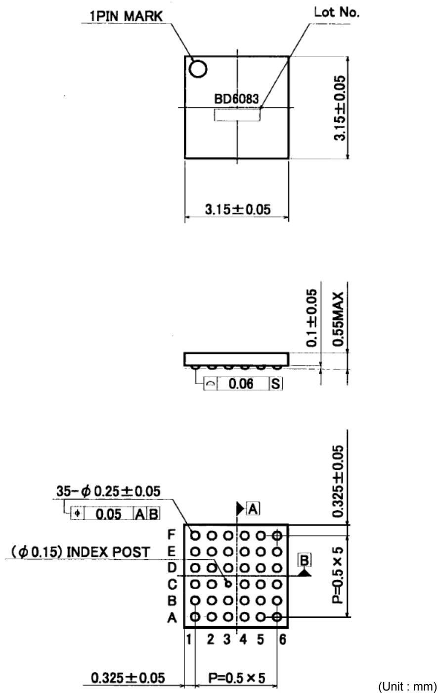
Fig.6 Package Outline
