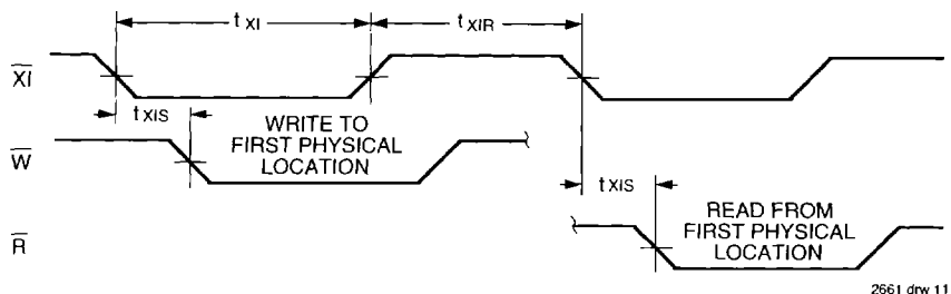
Figure 11. Expansion In
