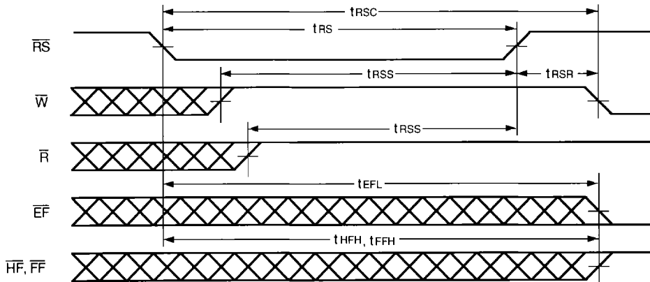
Figure 2. Reset
