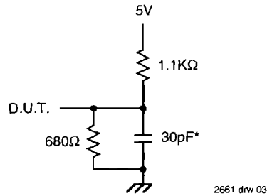
Figure 1. Output Load
