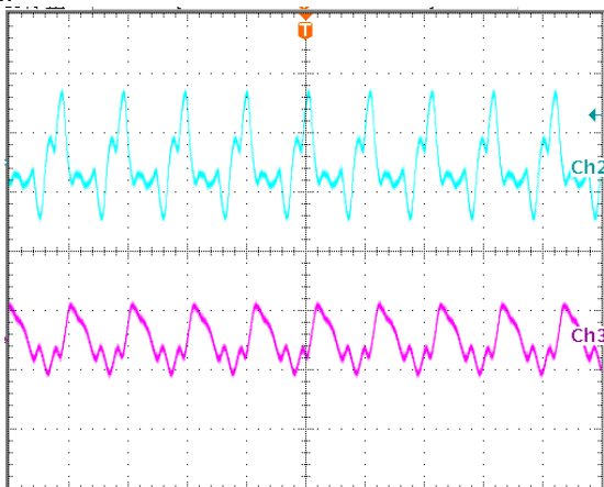
Output voltage ripple at nominal input voltage and max load current Top trace +12V, 10mV/div, Bottom trace -12V, 20mV/div, 2 \mu s/div. Load cap: 10 \mu F, tantalum capacitor and 1 \mu F ceramic capacitor. Bandwidth: 20MHz.
