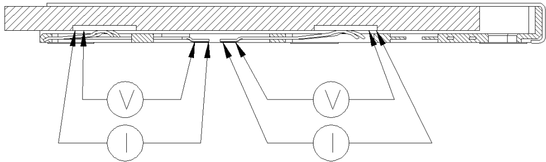
Fig.4 Measurement points of contact resistance
