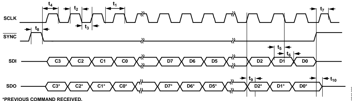
Figure 4. SPI Serial Interface Timing Diagram, CPOL = 0, CPHA = 1
