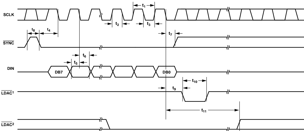
Figure 2. Timing Diagram
