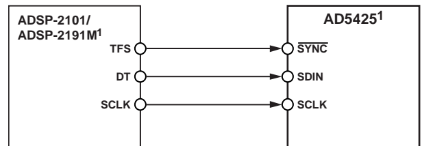
Figure 39. ADSP-2101/ADSP-2191M SPORT-to-AD5425 Interface
