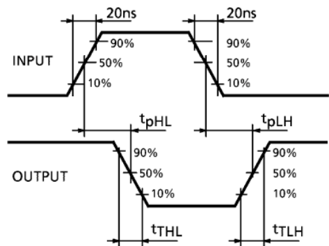
WAVEFORM
