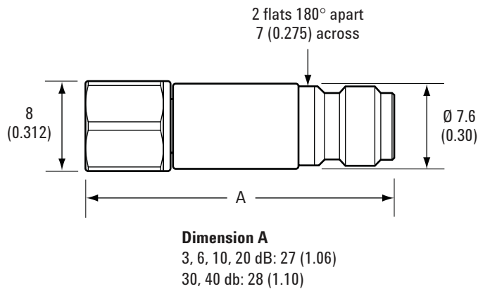
Figure 1. 8490G product outline
