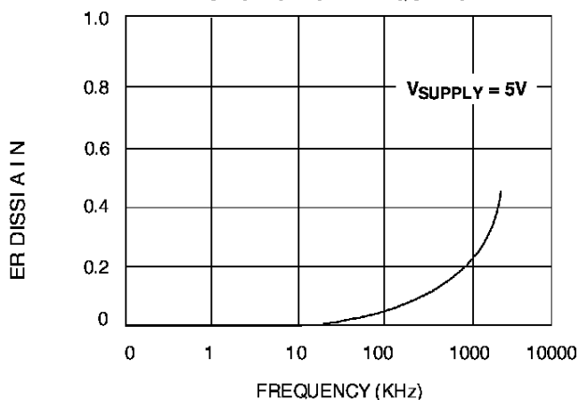
POWER DISSIPATION AS A FUNCTION OF FREQUENCY
