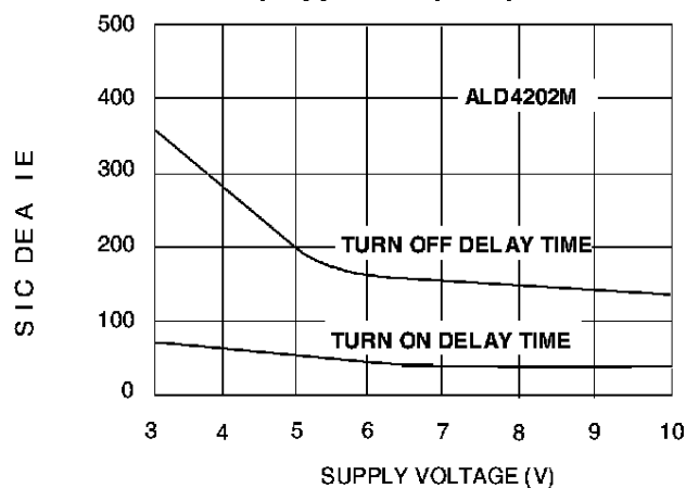
SWITCH DELAY TIME AS A FUNCTION OF SUPPLY VOLTAGE
