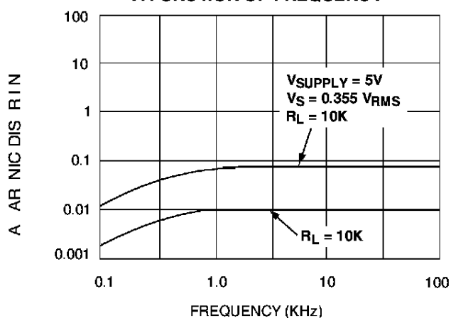
TOTAL HARMONIC DISTORTION AS A FUNCTION OF FREQUENCY
