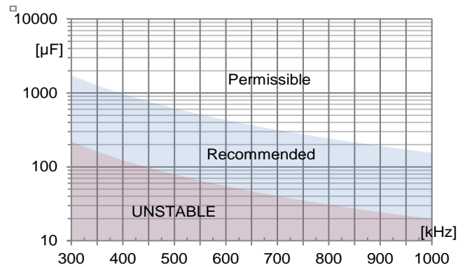
Effective total output capacitance limits vs switching frequency.
