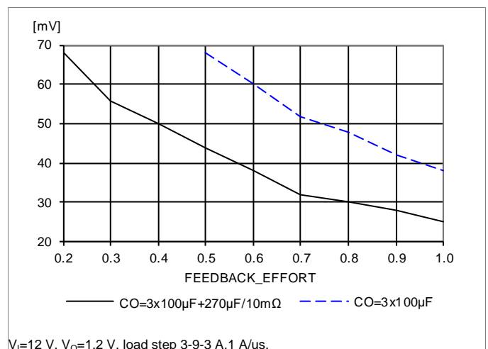
Voltage deviation vs. FEEDBACK_EFFORT setting.
