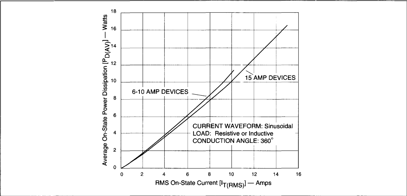
Figure 3.11 Power Dissipation (Typical) vs. On-State Current (6-10 and 15 Amp)
