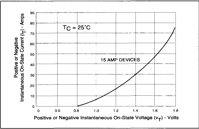
Figure 3.5 On-State Current vs On-State Voltage (Typical) (15 Amp)
