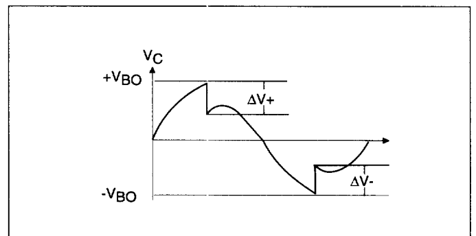
Figure 3.3 Test Circuit Waveforms
