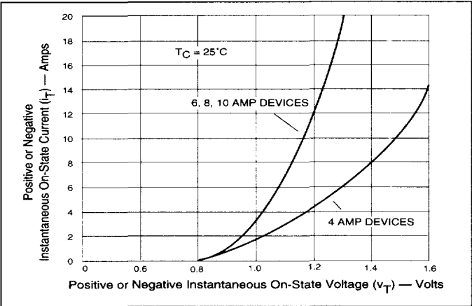
Figure 3.4 On-State Current vs On-State Voltage (Typical) (4-10 Amp)
