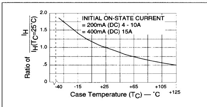
Figure 3.1 Normalized DC Holding Current vs Case Temperature
