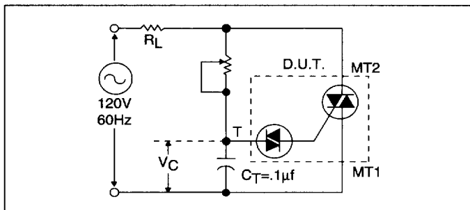
Figure 3.2 Test Circuit
