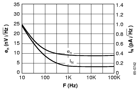
Figure 5. Input Noise Voltage, Current Density vs. Frequency
