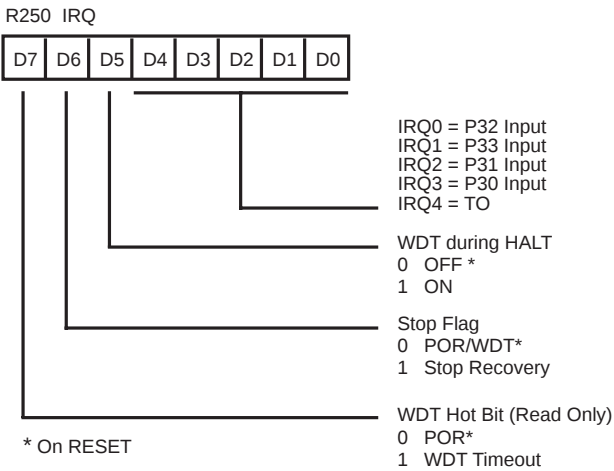
Figure 19. IRQ Register
