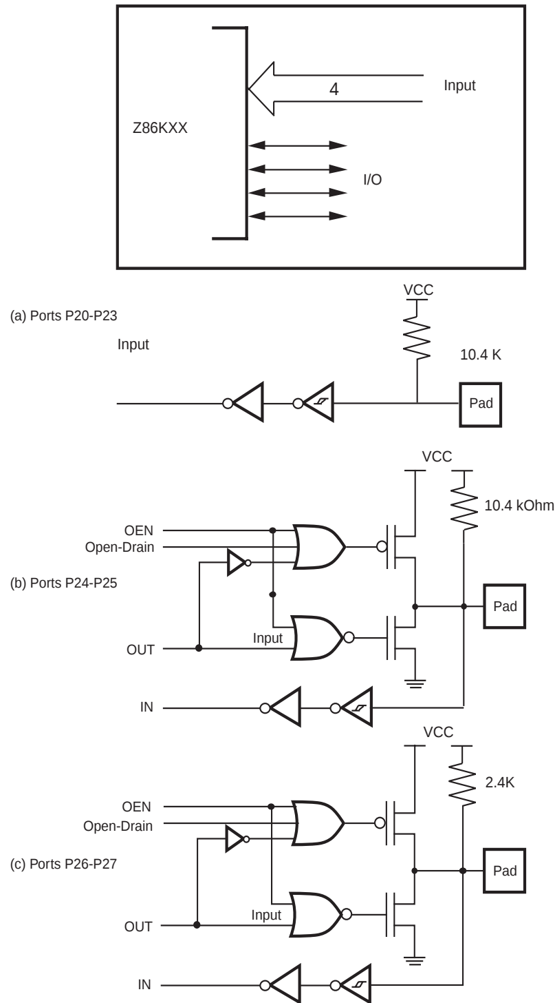
Figure 9. Port 2 Configuration
