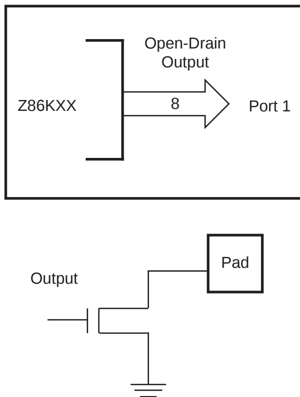
Figure 8. Port 1 Configuration
