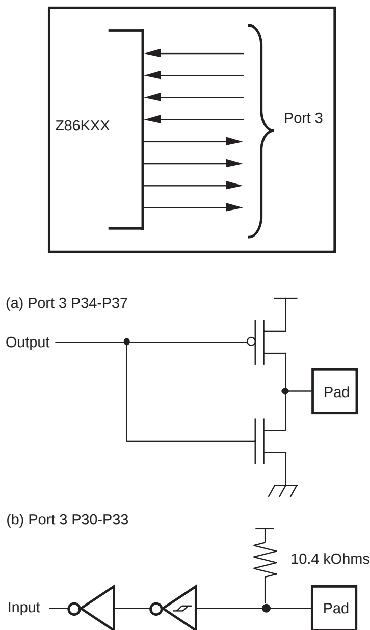
Figure 10. Port 3 Configuration
