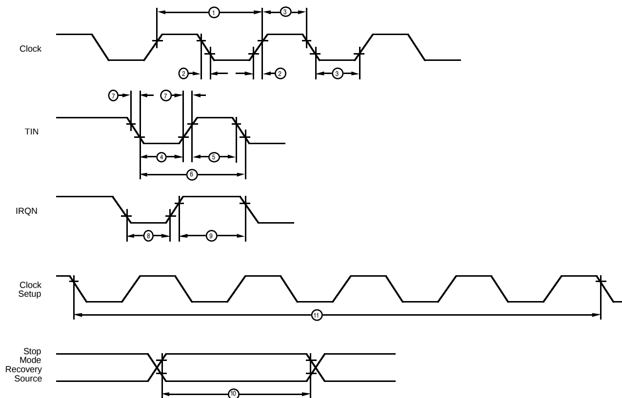
Figure 6. Additional Timing
