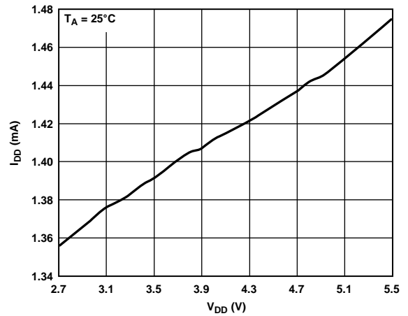
Figure 36. Supply Current vs. Supply Voltage
