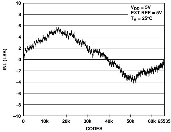
Figure 7. INL AD5668—External Reference
