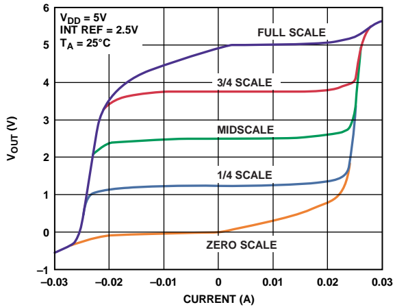
Figure 32. AD5668-2/AD5668-3 Source and Sink Capability
