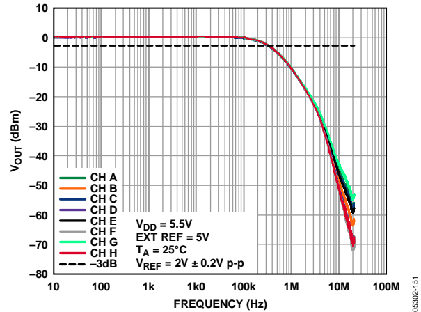
Figure 52. Multiplying Bandwidth
