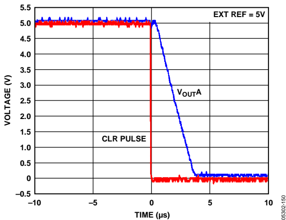
Figure 51. Hardware CLR
