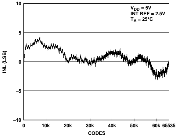
Figure 13. INL AD5668-2/AD5668-3
