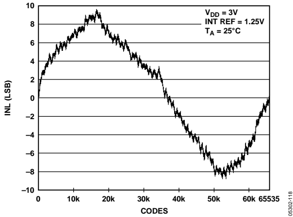
Figure 19. INL AD5668-1
