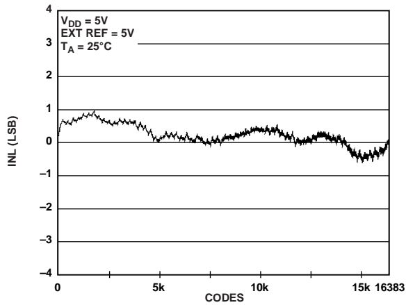
Figure 14. INL AD5648-2
