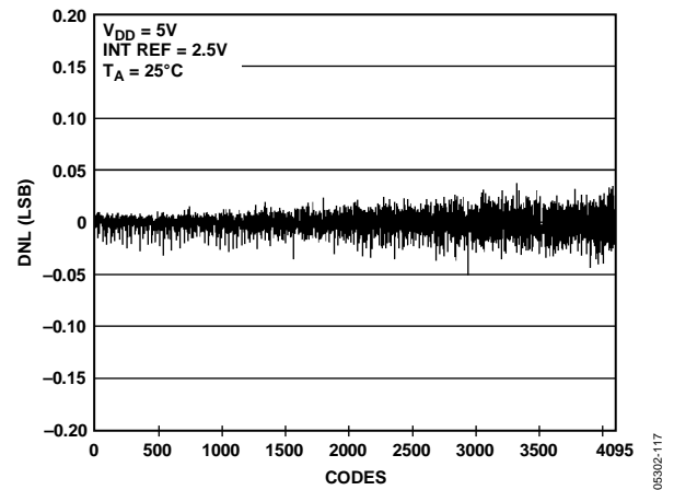
Figure 18. DNL AD5628-2
