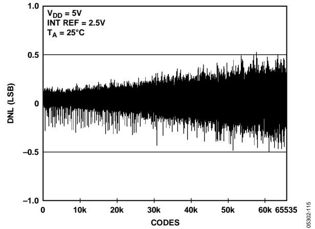
Figure 16. DNL AD5668-2/AD5668-3
