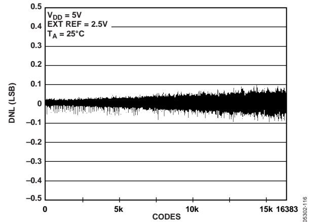
Figure 17. DNL AD5648-2
