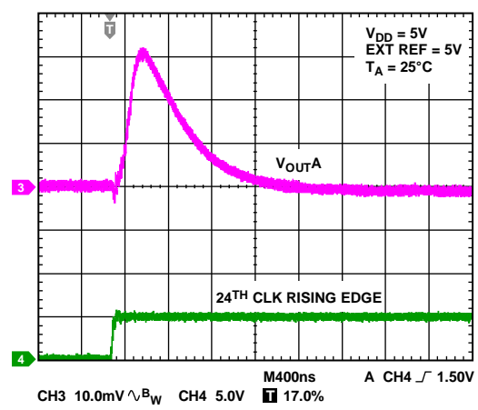
Figure 42. Digital-to-Analog Glitch Impulse (Negative)
