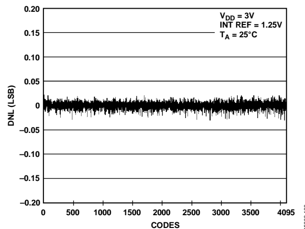
Figure 24. DNL AD5628-1
