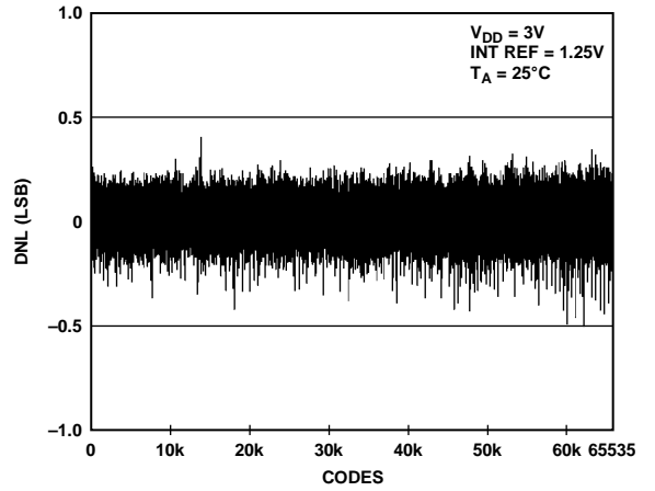
Figure 22. DNL AD5668-1
