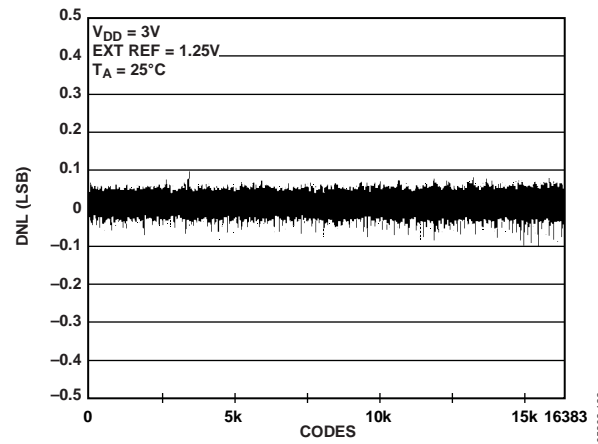
Figure 23. DNL AD5648-1
