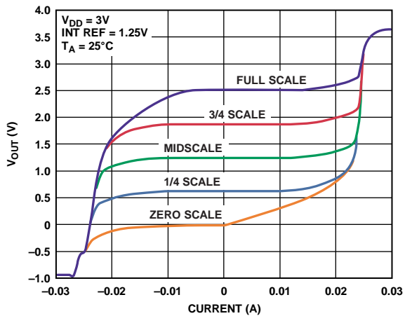
Figure 33. AD5668-1 Source and Sink Capability
