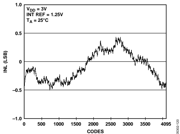
Figure 21. INL AD5628-1
