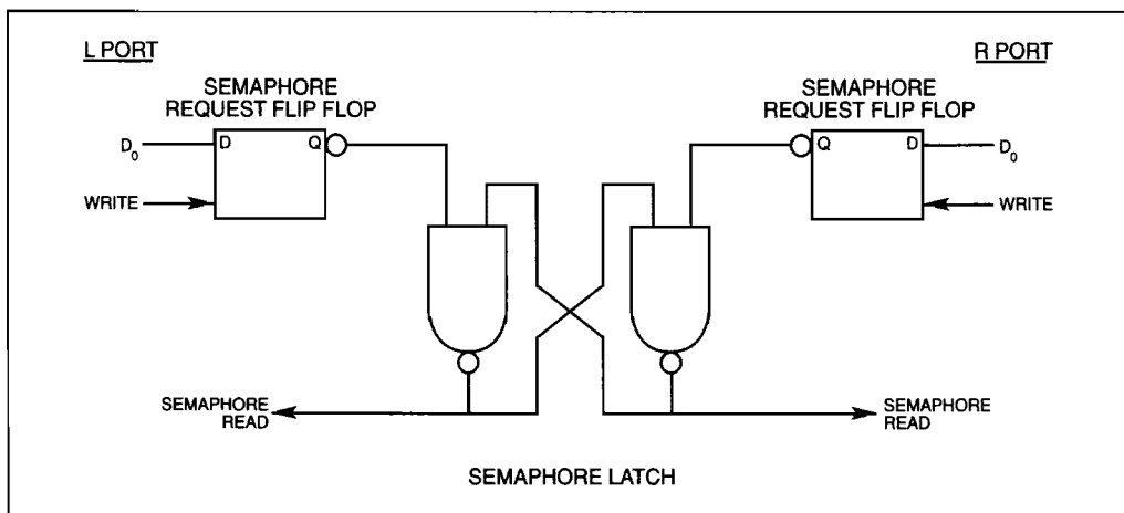
Figure 2 : M 67005 - Semaphore Logic.
