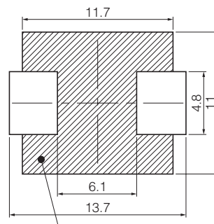
Series PCC-M1054M Series PCC-M1050M (ETQP5M□□□YFC/YGC)
