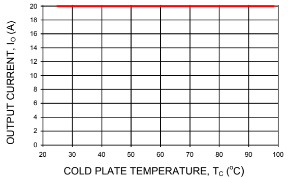
Figure 15. Output Current Derating for the Module in Conduction Cooling (cold plate) Applications, with or without Heatplate; T_a < 70^{\circ}\text{C} in vicinity of module interior; V_{IN} = 48\text{V} .
