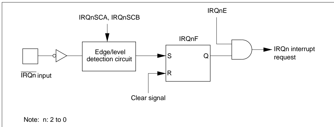
Figure 5.2 Block Diagram of Interrupts \overline{\text{IRQ2}} to \overline{\text{IRQ0}}
