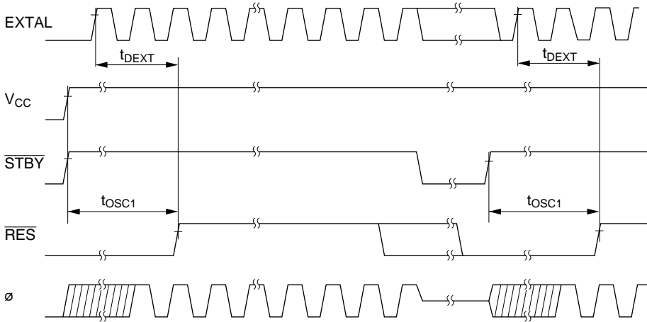
Figure 22.5 Oscillation Settling Timing
