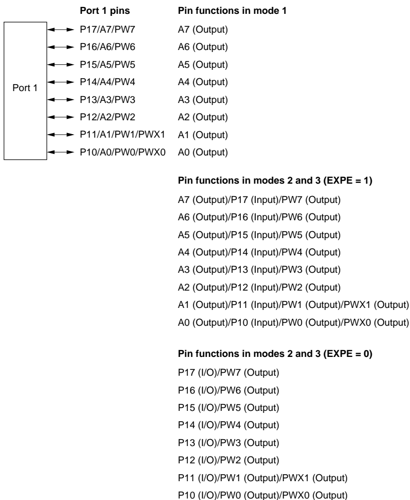
Figure 8.1 Port 1 Pin Functions
