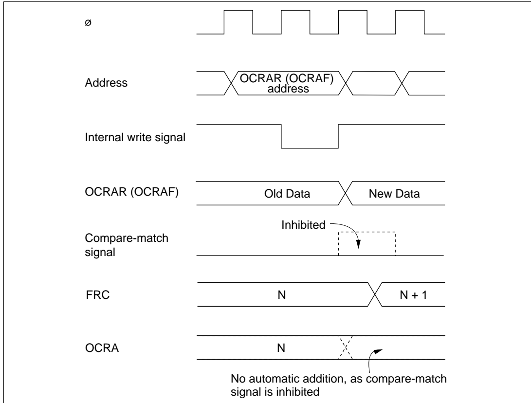
Figure 11.21 Contention between OCRAR/OCRAF Write and Compare-Match (When Automatic Addition Function Is Used)
