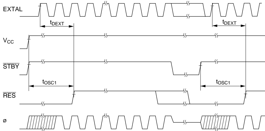
Figure 23.5 Oscillation Settling Timing
